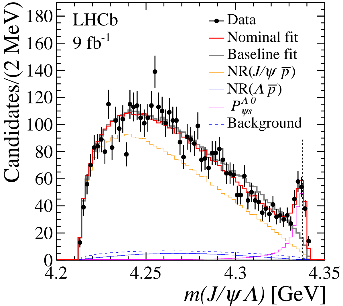
Figure 84.3: Distribution of invariant J/\psi \Lambda mass, with the projection of the amplitude fit model superimposed. The model without the P_{cs}(4338)^0 state (labeled as P_{\psi s}^{\Lambda 0} ) is also shown in grey. The \Xi_c^+ D^- baryon-meson threshold is indicated with a vertical dashed line.
