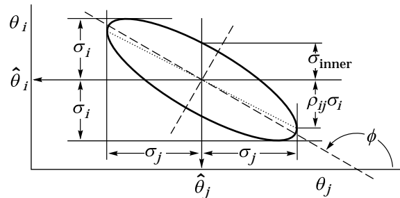
Figure 28.5: Standard error ellipse for the estimators \hat{\theta}_i and \hat{\theta}_j . In this case the correlation is negative.
