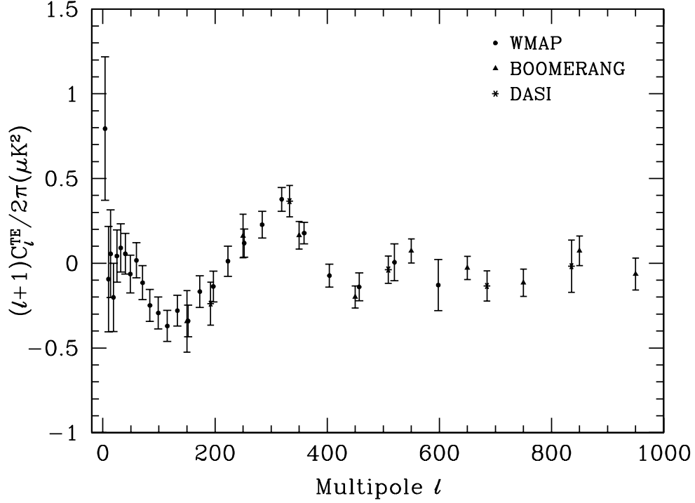
Figure 23.3: Cross power spectrum of the temperature anisotropies and E-mode polarization signal from WMAP [47], together with estimates from DASI and BOOMERANG which extend to higher \ell . Note that the BOOMERANG bands are wider in \ell than those of WMAP , while those of DASI are almost as wide as the features in the power spectrum. Also note that the y -axis here is not multiplied by the additional \ell , which helps to show both the large and small angular scale features.
