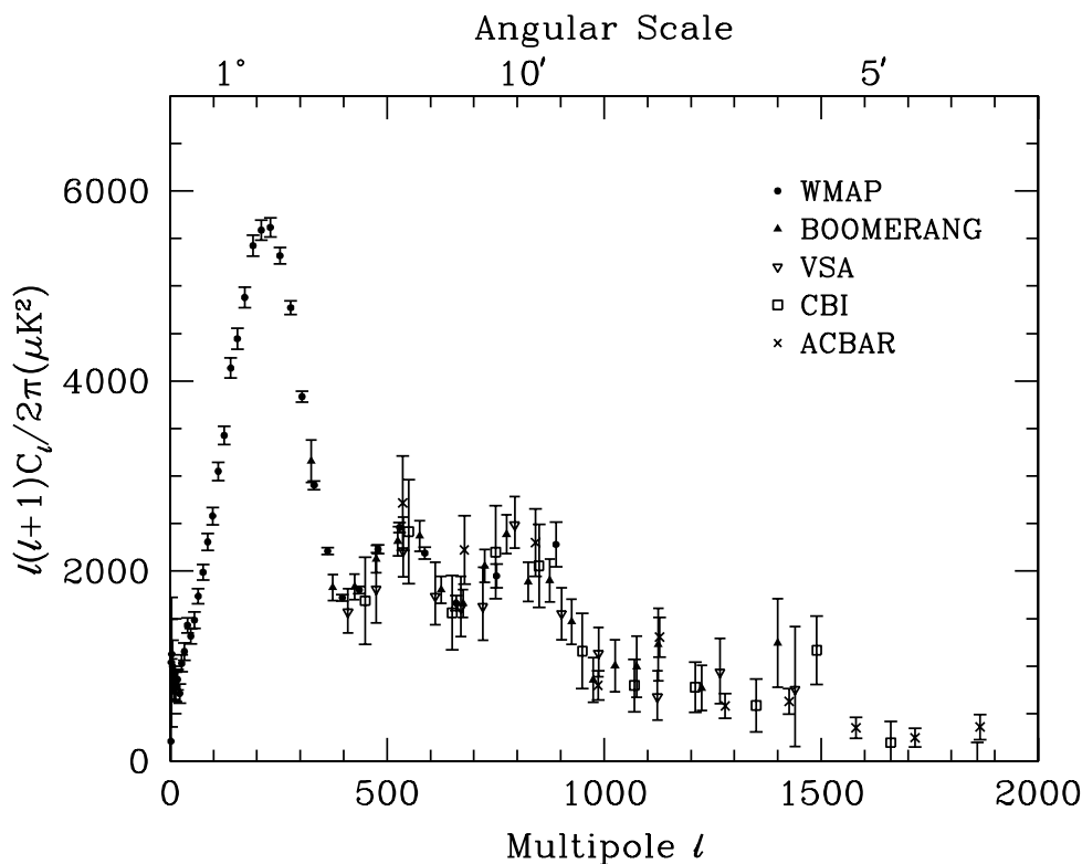
Figure 23.2: Band-power estimates from the WMAP , BOOMERANG , VSA , CBI , and ACBAR experiments. We have suppressed some of the low- \ell and high- \ell band-powers which have large error bars. Note also that the widths of the \ell -bands varies between experiments. This plot represent only a selection of available experimental results, with some other data-sets being of similar quality. The multipole axis here is linear, so the Sachs-Wolfe plateau is hard to see. However, the acoustic peaks and damping region are very clearly observed, with no need for a theoretical curve to guide the eye.
