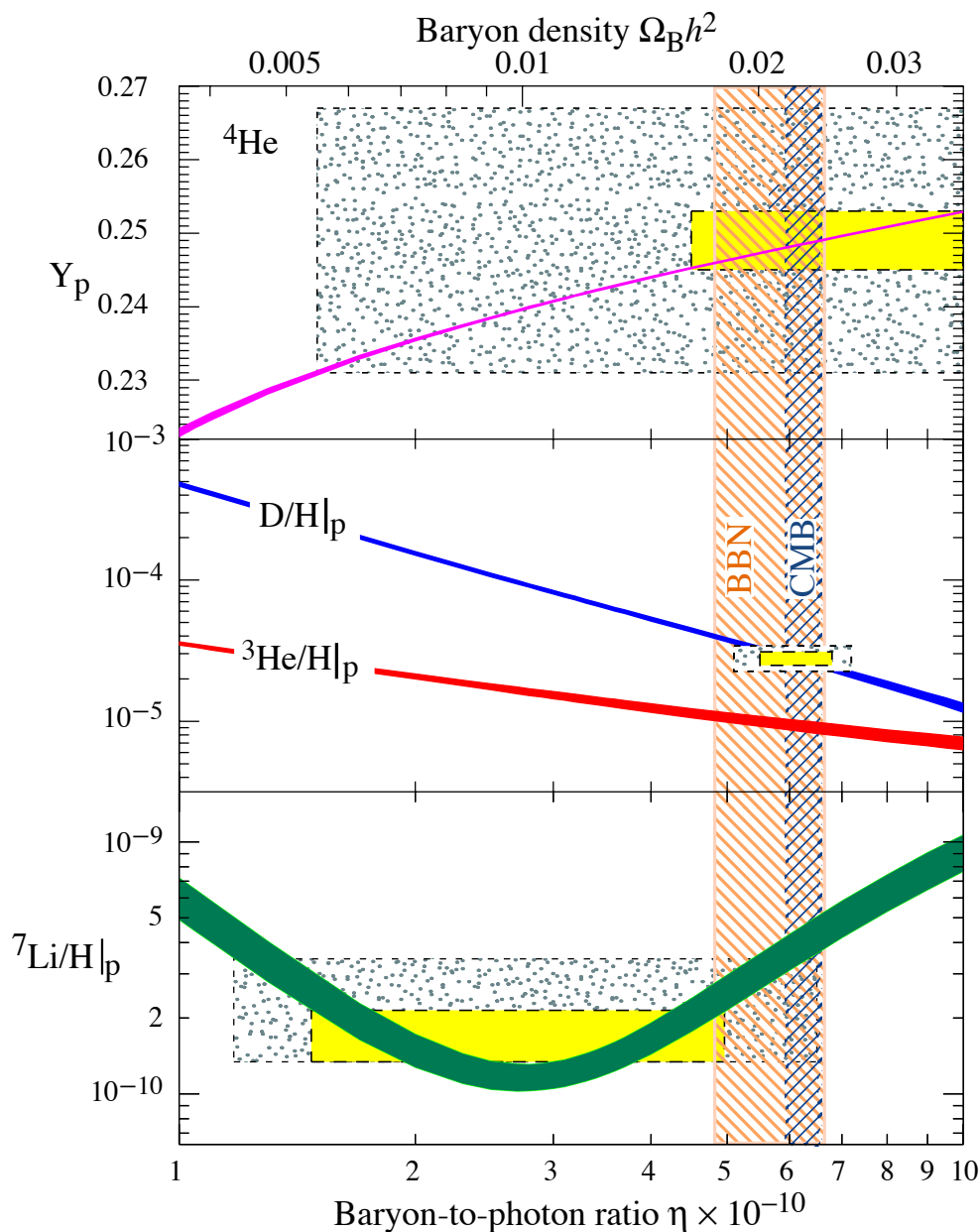
Figure 20.1: The abundances of {}^4\text{He} , D, {}^3\text{He} and {}^7\text{Li} as predicted by the standard model of big-bang nucleosynthesis — the bands the 95% CL range. Boxes indicate the observed light element abundances (smaller boxes: \pm 2\sigma statistical errors; larger boxes: \pm 2\sigma statistical and systematic errors). The narrow vertical band indicates the CMB measure of the cosmic baryon density, while the wider band indicates the BBN concordance range (both at 95% CL). Color version at end of book.
