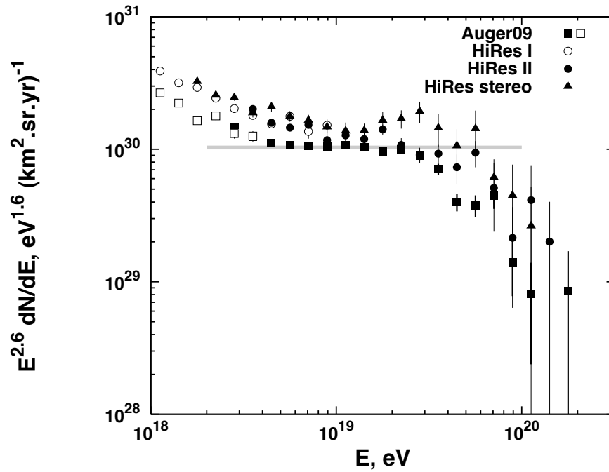
Figure 24.9: Expanded view of the highest energy portion of the cosmic-ray spectrum from data of the Auger Observatory (hybrid events shown with empty squares and HiRes in monocular and stereo modes). The differential cosmic ray flux is multiplied by E^{2.6} .
