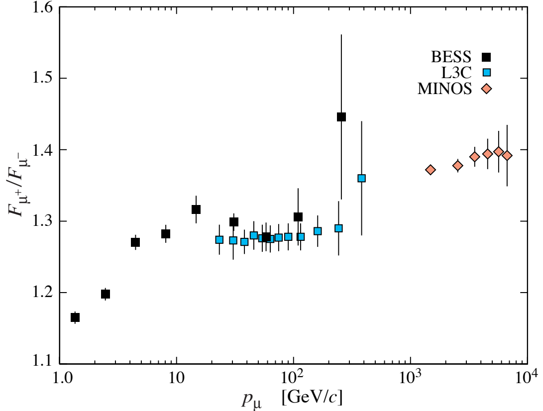
Figure 24.5: Muon charge ratio as a function of the muon momentum from Refs. [41,42,48].
