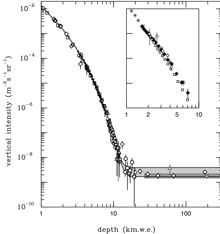
Figure 24.6: Vertical muon intensity vs depth ( 1 \text{ km.w.e.} = 10^5 \text{ g cm}^{-2} of standard rock). The experimental data are from: \diamond : the compilations of Crouch [55], \square : Baksan [60], \circ : LVD [61], \bullet : MACRO [62], \blacksquare : Frejus [63], and \triangle : SNO [64]. The shaded area at large depths represents neutrino-induced muons of energy above 2 GeV. The upper line is for horizontal neutrino-induced muons, the lower one for vertically upward muons. Darker shading shows the muon flux measured by the SuperKamiokande experiment.
