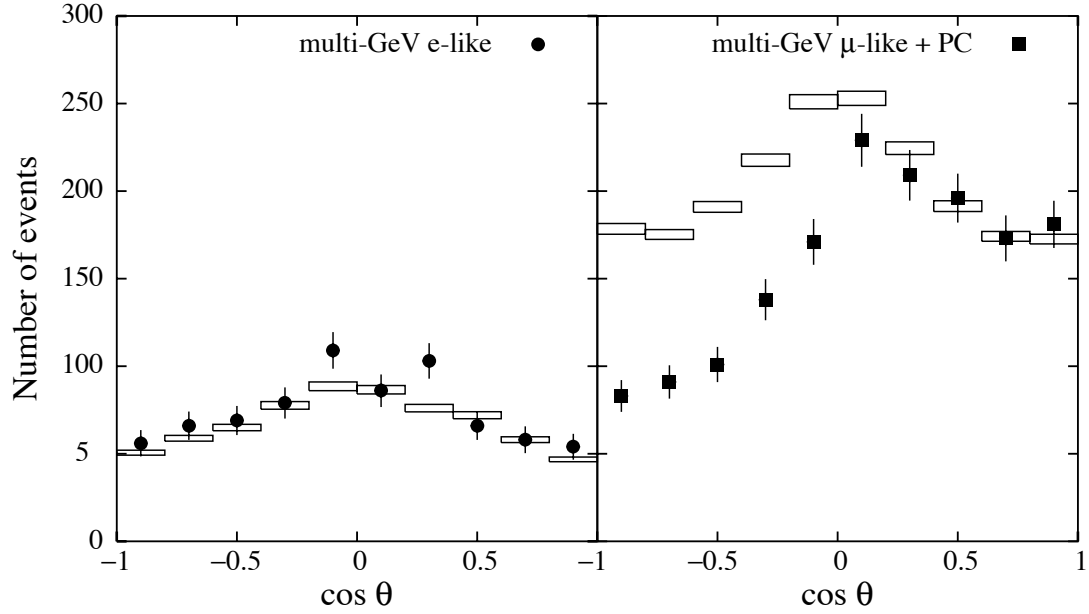
Figure 24.7: Zenith-angle dependence of multi-GeV neutrino interactions from SuperKamiokande [65]. The shaded boxes show the expectation in the absence of any oscillations.
