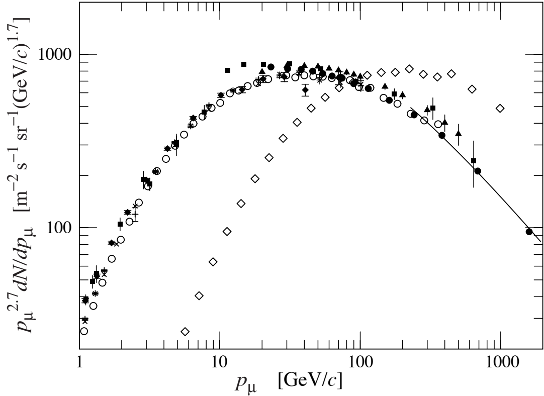
Figure 24.4: Spectrum of muons at \theta = 0^\circ ( \diamond [38], \blacksquare [43], \blacktriangledown [44], \blacktriangle [45], \times , + [40], \circ [41], and \bullet [42] and \theta = 75^\circ \diamond [46]). The line plots the result from Eq. (24.4) for vertical showers.
