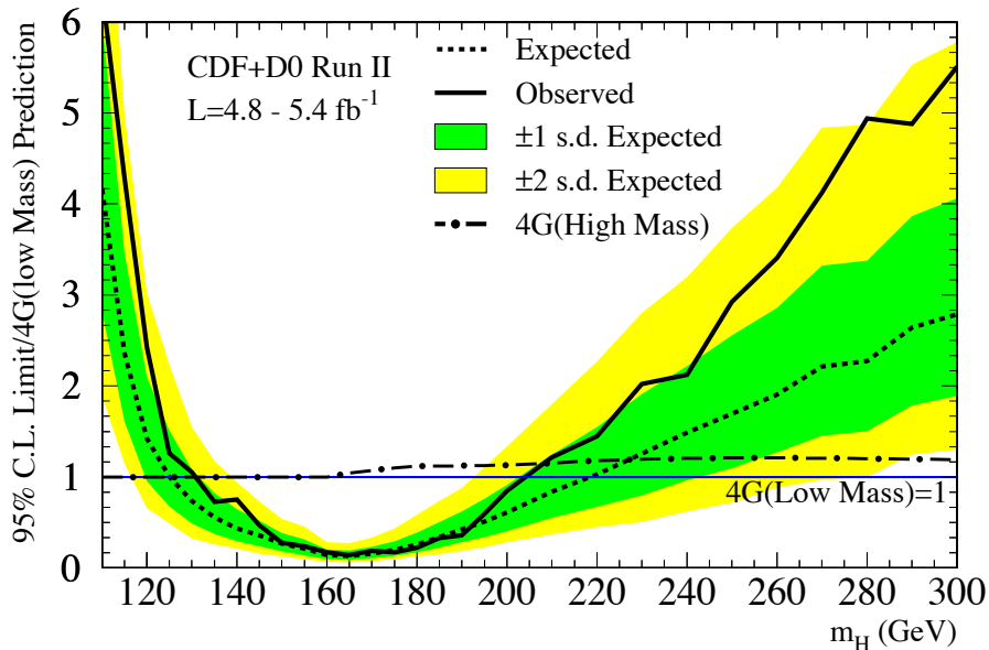
Figure 8: Upper bound on the Higgs boson cross section of the 4 th generation sequential model obtained by combining CDF and DØ search results in the H \rightarrow W^+W^- decay mode, as a function of the mass of the Higgs boson sought [87]. The limits are shown as a multiple of the cross section obtained in this extended model. The solid curve shows the observed upper bound, the dashed black curve shows the median expected upper bound assuming no signal is present, and the colored bands show the 68% and 95% probability bands around the expected upper bound. Color version at end of book.
