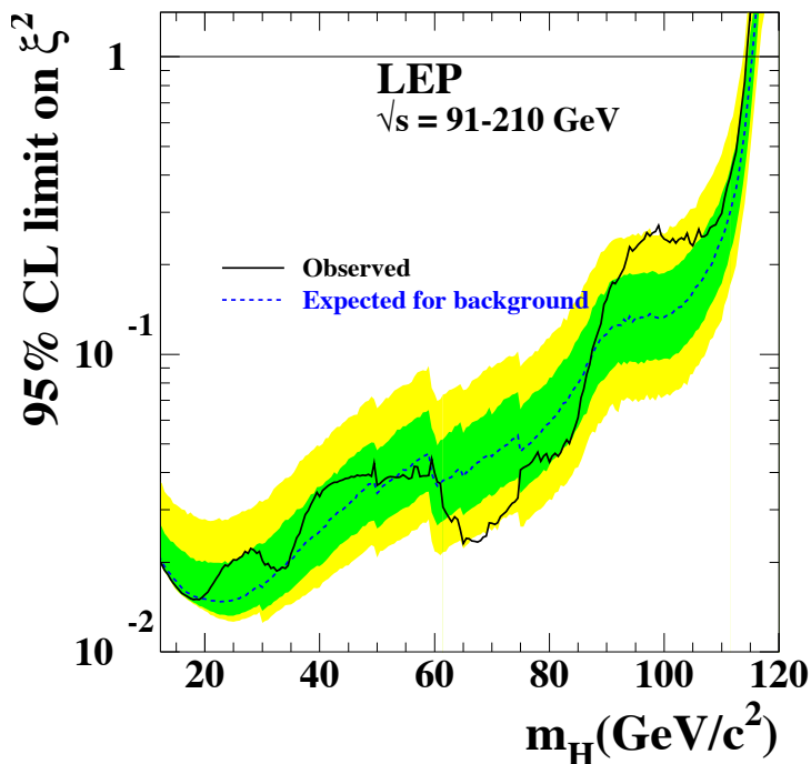
Figure 5: The 95% confidence level upper bound on the ratio \xi^2 = (g_{\text{HZZ}}/g_{\text{HZZ}}^{\text{SM}})^2 [17]. The solid line indicates the observed limit, and the dashed line indicates the median limit expected in the absence of a Higgs boson signal. The dark and light shaded bands around the expected limit line correspond to the 68% and 95% probability bands, indicating the range of statistical fluctuations of the expected outcomes. The horizontal line corresponds to the Standard Model coupling. Standard Model Higgs boson decay branching fractions are assumed. Color version at end of book.
