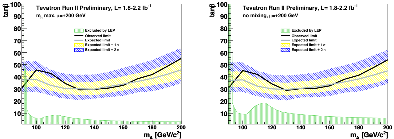
Figure 11: The 95% C.L. MSSM exclusion contours obtained by a combination of the CDF and D\bar{O} searches for H \rightarrow \tau^+\tau^- in the m_h -max (left) and no-mixing (right) benchmark scenarios, both with \mu = 200 GeV, projected onto the (m_A, \tan\beta) plane [147]. The regions above the solid black line are excluded, and the shaded and hatched bands centered on the lighter line show the distributions of expected exclusions in the absence of a signal. Also shown are the regions excluded by LEP searches [18], assuming a top quark mass of 174.3 GeV. The Tevatron results are not sensitive to the precise value of the top quark mass. Color version at end of book.
