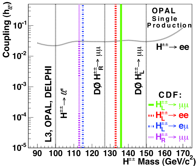
Figure 14: The 95% C.L. exclusion limits on the masses and couplings to leptons of right- and left-handed doubly-charged Higgs bosons, obtained by LEP and Tevatron experiments (from Ref. 223). Color version at end of book.
