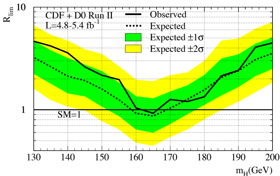
Figure 7: Upper bound on the SM Higgs boson cross section obtained by combining CDF and DØ search results in the H \rightarrow W^+W^- decay mode, as a function of the mass of the Higgs boson sought [19]. The limits are shown as a multiple of the SM cross section. The ratios of the different production and decay modes are assumed to be as predicted by the SM. The solid curve shows the observed upper bound, the dashed black curve shows the median expected upper bound assuming no signal is present. The shaded bands show the 68% and 95% probability bands around the expected upper bound. Color version at end of book.
