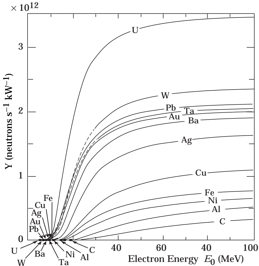
Figure 30.1: Neutron yields from semi-infinite targets per kW of electron beam power, as a function of the electron beam energy, disregarding target self-shielding [5].
