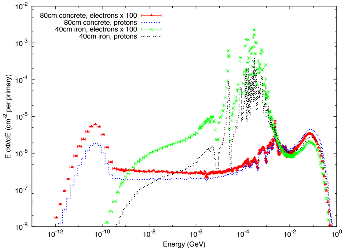
Figure 30.2: Neutron energy spectra calculated with the FLUKA code [6,7] from 25 GeV proton and electron beams on a thick copper target. Spectra are evaluated at 90^\circ to the beam direction behind 80 cm of concrete or 40 cm of iron. All spectra are normalized per beam particle. In addition, spectra for electron beam are multiplied by a factor of 100. See full-color version on color pages at end of book.
