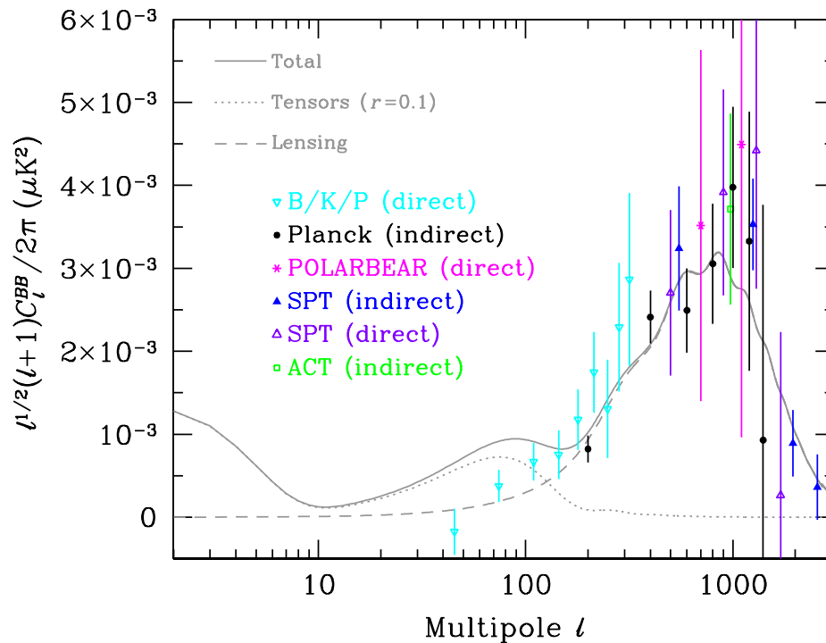
Figure 27.5: Power spectrum of B -mode polarization, including results from the BICEP2/Keck Array/ Planck combined analysis (B/K/P), Planck , POLARBEAR, SPT, and ACT. Note that some of the measurements are direct estimates of B -modes on the sky, while others are only sensitive to the lensing signal and come from combining E -mode and lensing potential measurements. Several experiments have previously reported upper limits, which are all off the top of this plot. A logarithmic x -axis is adopted here and the y -axis has been divided by a factor of \sqrt{\ell} in order to show all three theoretically expected contributions: the low- \ell reionization bump; the \ell \sim 100 recombination peak; and the high- \ell lensing signature. The dotted line is for a tensor (primordial gravitational wave) fraction r = 0.1 , simply as an example, with all other cosmological parameters set at the best Planck -derived values, for which model the expected lensing B -modes have also been shown with a dashed line.
