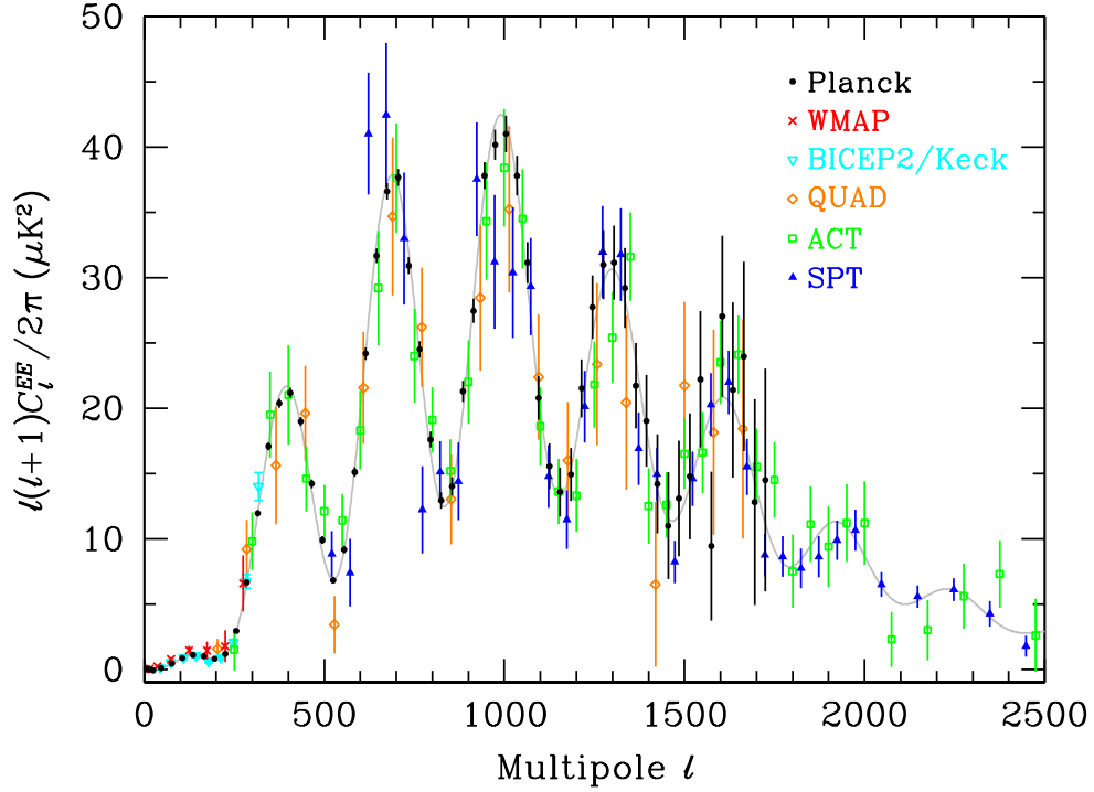
Figure 27.4: Power spectrum of E -mode polarization from Planck , together with WMAP , BICEP2/Keck , QUAD , ACT , and SPT . Note that some band-powers with larger uncertainties have been omitted and that the unbinned Planck low- \ell data have been binned here. Also plotted is the best-fit theoretical model from Planck TT data (plus polarization at \ell < 30 and CMB lensing).
