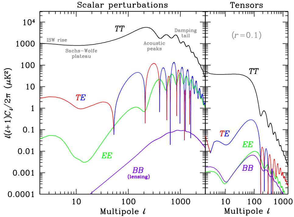
Figure 27.1: Theoretical CMB anisotropy power spectra, using the best-fitting \Lambda CDM model from Planck , calculated using CAMB. The panel on the left shows the theoretical expectation for scalar perturbations, while the panel on the right is for tensor perturbations with an amplitude set to r = 0.1 . Note that the x -axis is logarithmic here. For the well-measured scalar TT spectrum, the regions, each covering roughly a decade in \ell , are labeled as in the text: the ISW rise; Sachs-Wolfe plateau; acoustic peaks; and damping tail. The TE cross-correlation power spectra change sign, and that has been indicated by plotting the absolute value, but switching color for the negative parts.
