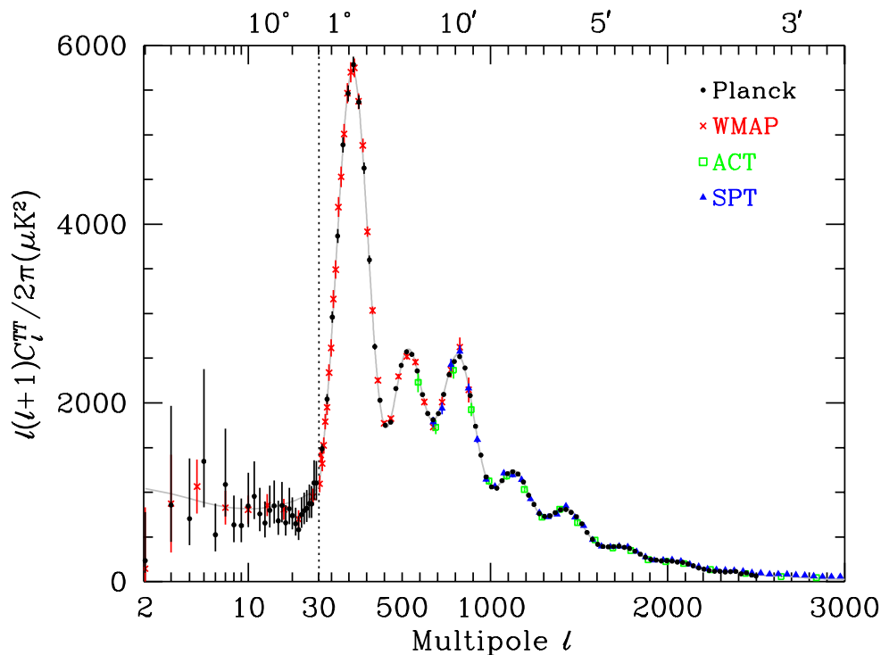
Figure 27.2: CMB temperature anisotropy band-power estimates from the Planck , WMAP , ACT , and SPT experiments. Note that the widths of the \ell -bands vary between experiments and have not been plotted. This figure represents only a selection of the most recent available experimental results, and some points with large error bars have been omitted. At the higher multipoles these band-powers involve subtraction of particular foreground models, while proper analysis requires simultaneous fitting of CMB and foregrounds over multiple frequencies. The x -axis here is logarithmic for the lowest multipoles, to show the Sachs-Wolfe plateau, and linear for the other multipoles. The acoustic peaks and damping region are very clearly observed, with no need for a theoretical curve to guide the eye; however, the curve plotted is the best-fit Planck model.
