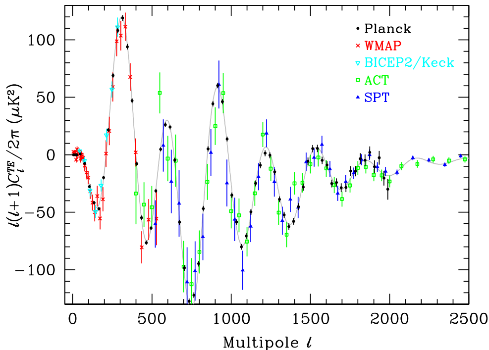
Figure 27.3: Cross-power spectrum band-powers of the temperature anisotropies and E -mode polarization signal from Planck (the low multipole data have been binned here), WMAP , BICEP2/Keck, ACT, and SPT. The curve is the prediction from the best fit to the Planck temperature band-powers (as well as the \ell < 30 polarization and CMB lensing results) and is not a fit to these data; however, these TE measurements follow the curve very closely, showing the expected oscillatory structure. Note that each band-power is an average over a range of multipoles, and hence to compare in detail with a model one has to average the theoretical curve through the band.
