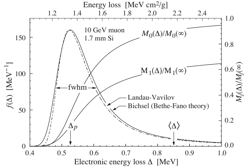
Figure 32.7: Electronic energy deposit distribution for a 10 GeV muon traversing 1.7 mm of silicon, the stopping power equivalent of about 0.3 cm of PVC scintillator [1,13,28]. The Landau-Vavilov function (dot-dashed) uses a Rutherford cross section without atomic binding corrections but with a kinetic energy transfer limit of W_{\text{max}} . The solid curve was calculated using Bethe-Fano theory. M_0(\Delta) and M_1(\Delta) are the cumulative 0th moment (mean number of collisions) and 1st moment (mean energy loss) in crossing the silicon. (See Sec. 32.2.1. The fwhm of the Landau-Vavilov function is about 4\xi for detectors of moderate thickness. \Delta_p is the most probable energy loss, and \langle\Delta\rangle divided by the thickness is the Bethe \langle dE/dx \rangle ).
