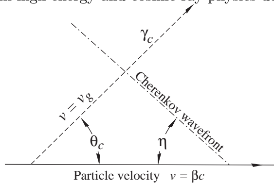
Figure 32.26: Cherenkov light emission and wavefront angles. In a dispersive medium, \theta_c + \eta \neq 90^\circ .
