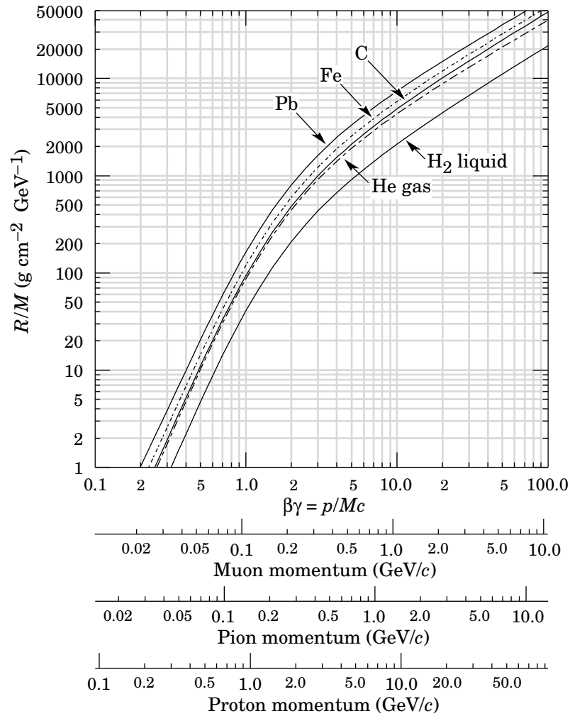
Figure 32.4: Range of heavy charged particles in liquid (bubble chamber) hydrogen, helium gas, carbon, iron, and lead. For example: For a K^+ whose momentum is 700 MeV/c, \beta\gamma = 1.42 . For lead we read R/M \approx 396 , and so the range is 195 \text{ g cm}^{-2} (17 cm).
