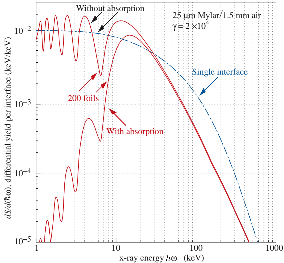
Figure 32.27: X-ray photon energy spectra for a radiator consisting of 200 25\ \mu\text{m} thick foils of Mylar with 1.5 mm spacing in air (solid lines) and for a single surface (dashed line). Curves are shown with and without absorption. Adapted from Ref. 88.
