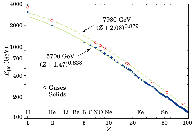
Figure 32.24: Muon critical energy for the chemical elements, defined as the energy at which radiative and ionization energy loss rates are equal [5]. The equality comes at a higher energy for gases than for solids or liquids with the same atomic number because of a smaller density effect reduction of the ionization losses. The fits shown in the figure exclude hydrogen. Alkali metals fall 3–4% above the fitted function, while most other solids are within 2% of the function. Among the gases the worst fit is for radon (2.7% high).
