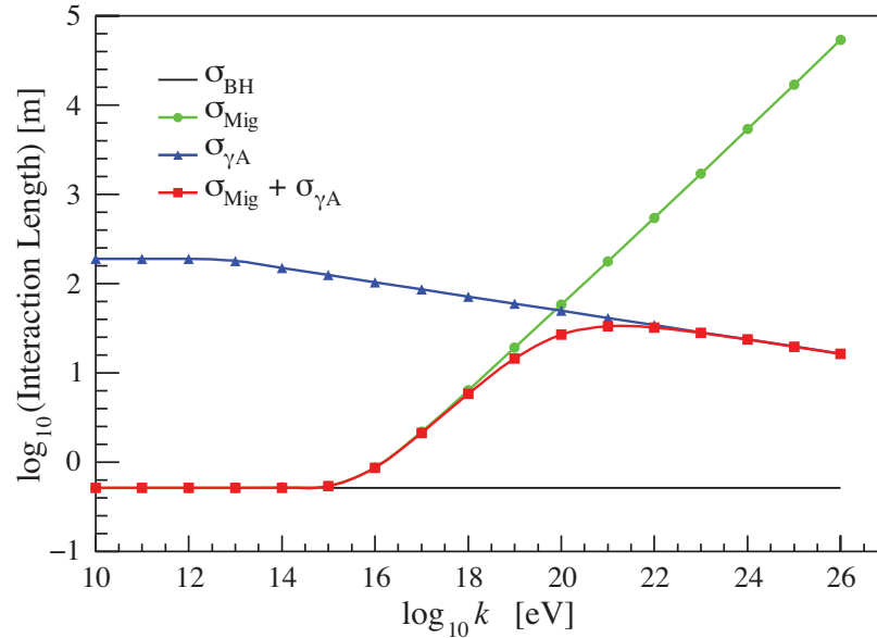
Figure 32.19: Interaction length for a photon in ice as a function of photon energy for the Bethe-Heitler (BH), LPM (Mig) and photonuclear ( \gamma A ) cross sections [56]. The Bethe-Heitler interaction length is 9X_0/7 , and X_0 is 0.393 m in ice.
