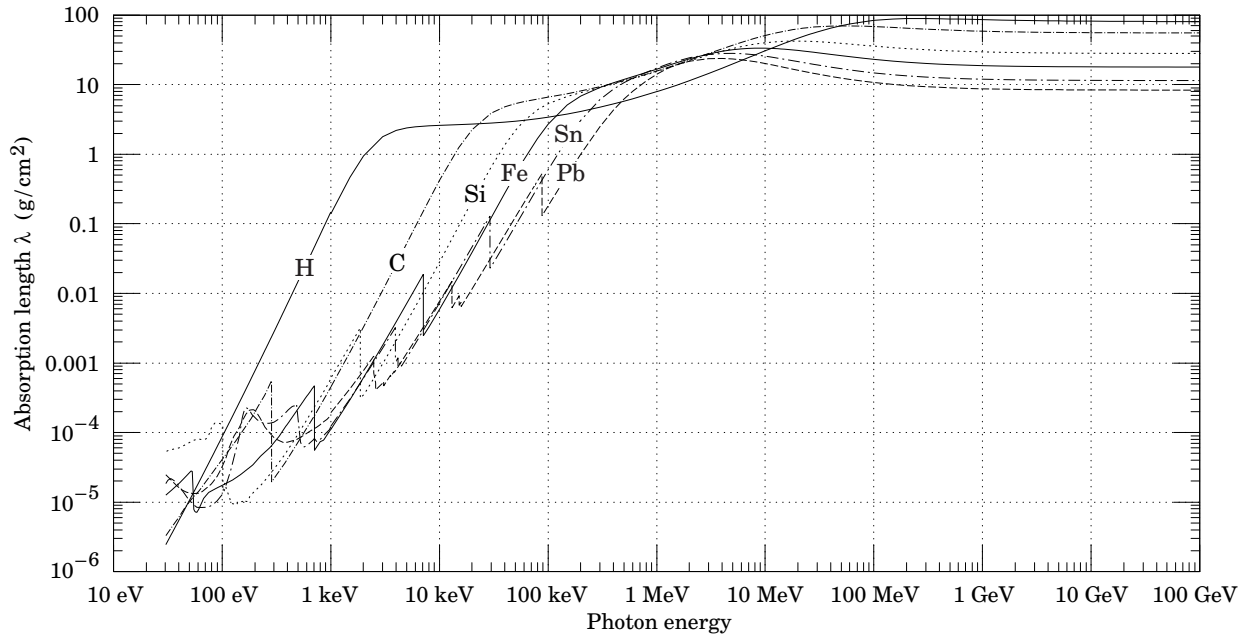
Figure 32.16: The photon mass attenuation length (or mean free path) \lambda = 1/(\mu/\rho) for various elemental absorbers as a function of photon energy. The mass attenuation coefficient is \mu/\rho , where \rho is the density. The intensity I remaining after traversal of thickness t (in mass/unit area) is given by I = I_0 \exp(-t/\lambda) . The accuracy is a few percent. For a chemical compound or mixture, 1/\lambda_{\text{eff}} \approx \sum_{\text{elements}} w_Z/\lambda_Z , where w_Z is the proportion by weight of the element with atomic number Z . The processes responsible for attenuation are given in Fig. 32.11. Since coherent processes are included, not all these processes result in energy deposition. The data for 30 \text{ eV} < E < 1 \text{ keV} are obtained from http://www-cxro.lbl.gov/optical_constants (courtesy of Eric M. Gullikson, LBNL). The data for 1 \text{ keV} < E < 100 \text{ GeV} are from http://physics.nist.gov/PhysRefData , through the courtesy of John H. Hubbell (NIST).
