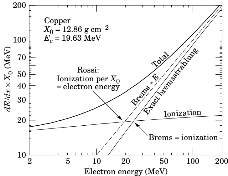
Figure 32.13: Two definitions of the critical energy E_c .
