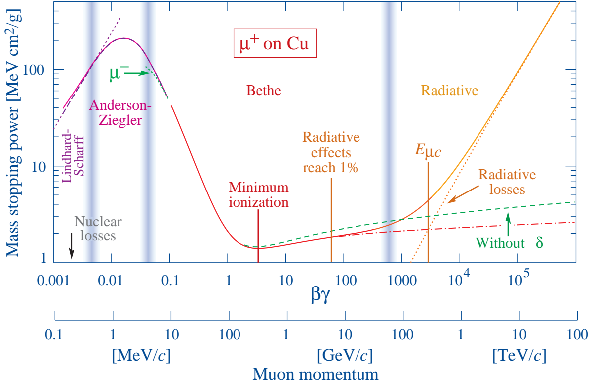
Fig. 32.1: Mass stopping power ( = \langle -dE/dx \rangle ) for positive muons in copper as a function of \beta\gamma = p/Mc over nine orders of magnitude in momentum (12 orders of magnitude in kinetic energy). Solid curves indicate the total stopping power. Data below the break at \beta\gamma \approx 0.1 are taken from ICRU 49 [4], and data at higher energies are from Ref. 5. Vertical bands indicate boundaries between different approximations discussed in the text. The short dotted lines labeled “ \mu^- ” illustrate the “Barkas effect,” the dependence of stopping power on projectile charge at very low energies [6]. dE/dx in the radiative region is not simply a function of \beta .
