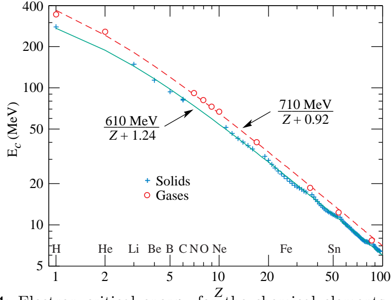
Figure 32.14: Electron critical energy for the chemical elements, using Rossi's definition [2]. The fits shown are for solids and liquids (solid line) and gases (dashed line). The rms deviation is 2.2% for the solids and 4.0% for the gases. (Computed with code supplied by A. Fassó.)
