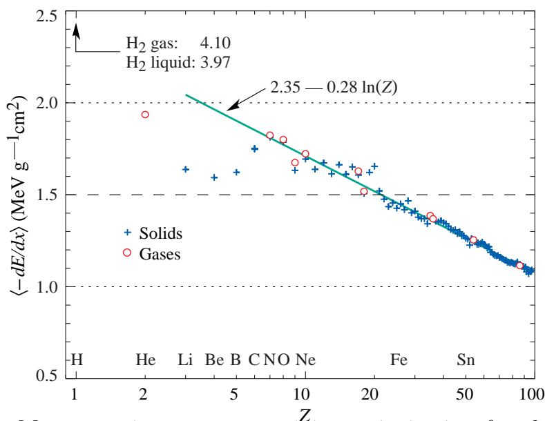
Figure 32.3: Mass stopping power at minimum ionization for the chemical elements. The straight line is fitted for Z > 6 . A simple functional dependence on Z is not to be expected, since \langle -dE/dx \rangle also depends on other variables.
