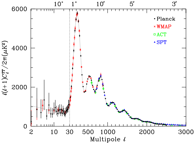
Figure 28.1: CMB temperature anisotropy band-power estimates from the Planck , WMAP , ACT, and SPT experiments.
