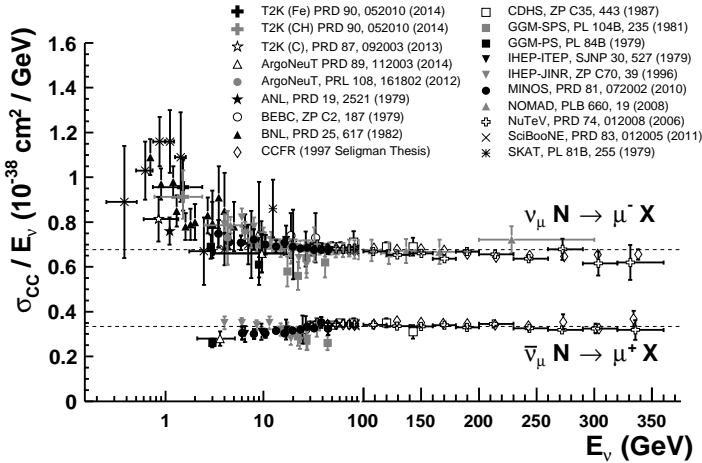
Figure 50.1: Measurements of \nu_\mu and \bar{\nu}_\mu CC inclusive scattering cross sections (per nucleon) divided by neutrino energy as a function of neutrino energy.
