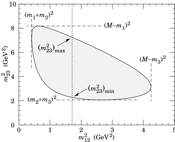
Figure 47.3: Dalitz plot for a three-body final state. In this example, the state is \pi^+K^0p at 3 GeV. Four-momentum conservation restricts events to the shaded region.
