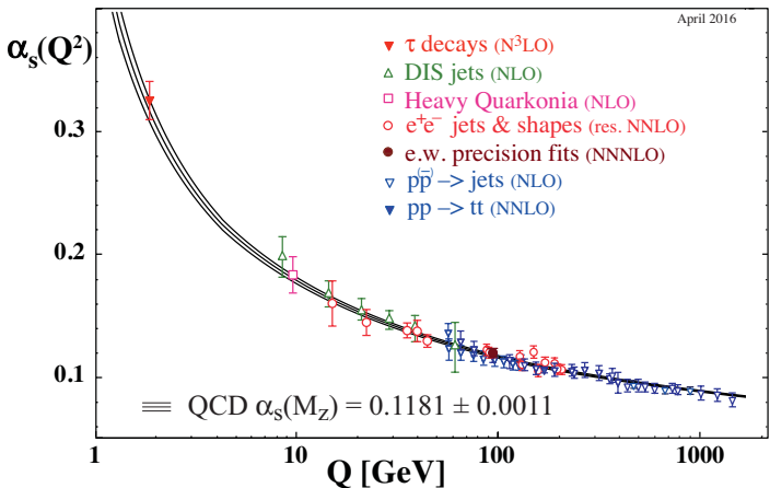
Figure 9.3: Summary of measurements of \alpha_s as a function of the energy scale Q .
