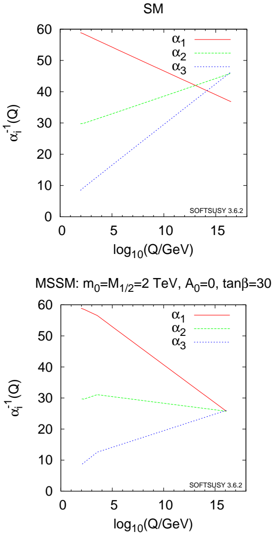
Figure 16.1: Running couplings in SM and MSSM using two-loop RG evolution. (We thank Ben Allanach for providing the plots created using SOFTSUSY.)
