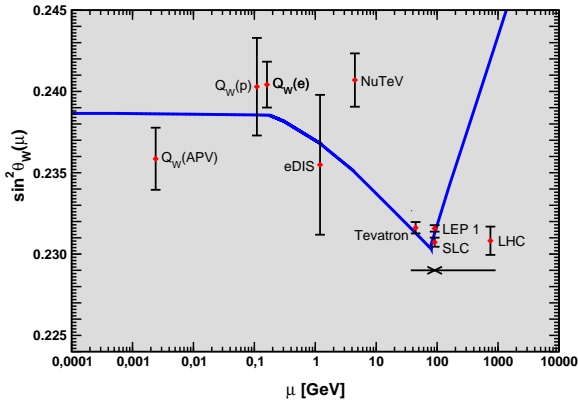
Figure 10.2: Scale dependence of the weak mixing angle in the \overline{\text{MS}} scheme [122]. The width of the curve reflects the theory uncertainty from strong interaction effects which at low energies is at the level of \pm 7 \times 10^{-5} [122]. For NuTeV we display the updated value from Ref. 125. The Tevatron and LHC measurements are strongly dominated by invariant masses of the final state dilepton pair of \mathcal{O}(M_Z) and can thus be considered as additional Z pole data points. For clarity we displayed the Tevatron and LHC points horizontally to the left and to the right, respectively.
