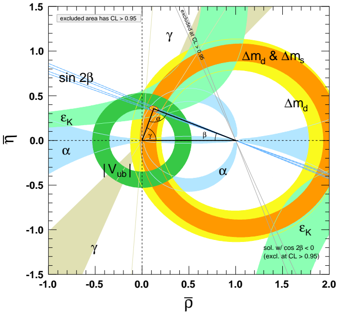
Figure 12.2: 95% CL constraints on the \bar{\rho}, \bar{\eta} plane.
