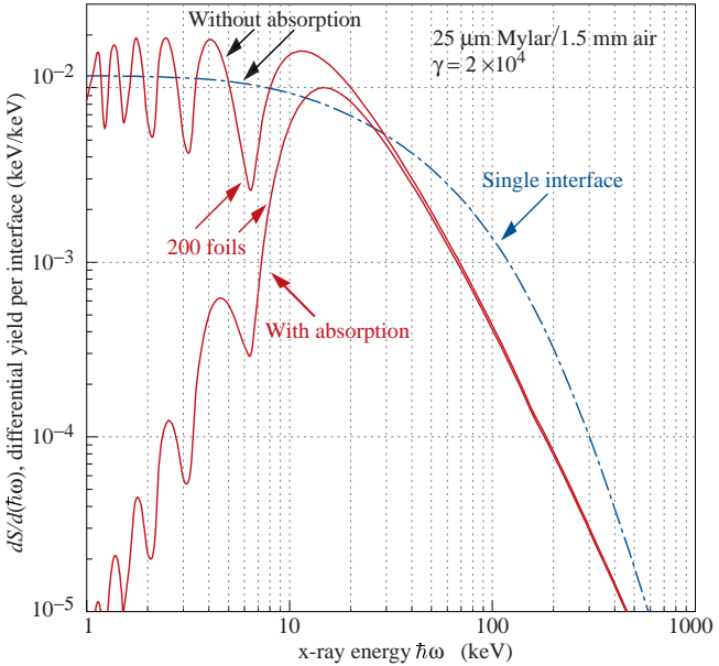
Figure 33.27: X-ray photon energy spectra for a radiator consisting of 200 25\ \mu\text{m} thick foils of Mylar with 1.5\ \text{mm} spacing in air (solid lines) and for a single surface (dashed line). Curves are shown with and without absorption. Adapted from Ref. 88.
