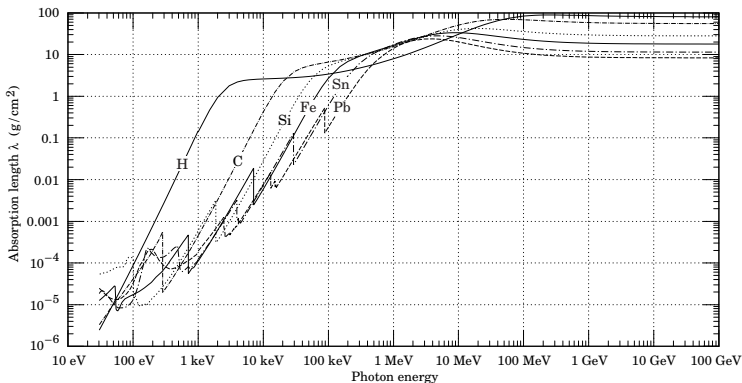
Fig. 33.16: The photon mass attenuation length (or mean free path) \lambda = 1/(\mu/\rho) for various elemental absorbers as a function of photon energy. The mass attenuation coefficient is \mu/\rho , where \rho is the density. The intensity I remaining after traversal of thickness t (in mass/unit area) is given by I = I_0 \exp(-t/\lambda) . The accuracy is a few percent. For a chemical compound or mixture, 1/\lambda_{\text{eff}} \approx \sum_{\text{elements}} w_Z/\lambda_Z , where w_Z is the proportion by weight of the element with atomic number Z . The processes responsible for attenuation are given in Fig. 33.11. Since coherent processes are included, not all these processes result in energy deposition.
