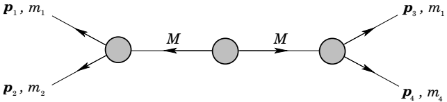
Figure 47.9: Definitions of variables for pair production of semi-invisible final states. Particles 1 and 3 are invisible while particles 2 and 4 are visible.
