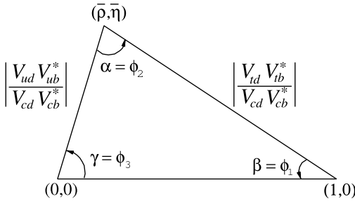
Figure 12.1: Sketch of the unitarity triangle.
