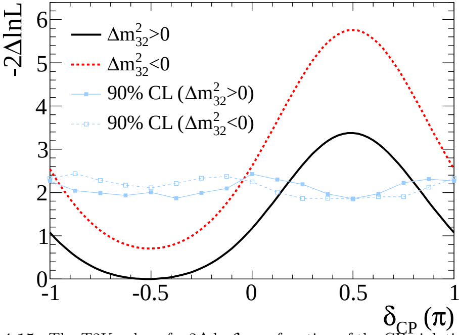
Figure 14.15: The T2K value of -2\Delta \ln \mathcal{L} as a function of the CP violating phase \delta for normal mass ordering (solid line) and inverted mass ordering (dotted line). The likelihood is marginalized over \sin^2 2\theta_{13} , \sin^2 \theta_{23} and \Delta m^2_{32} . The solid (dotted) line with markers corresponds to the 90% CL limits for normal (inverted) mass ordering, evaluated by using the Feldman-Cousins method. The \delta regions with values above the lines are excluded at 90% CL. This figure is taken from arXiv:1311.4750.
