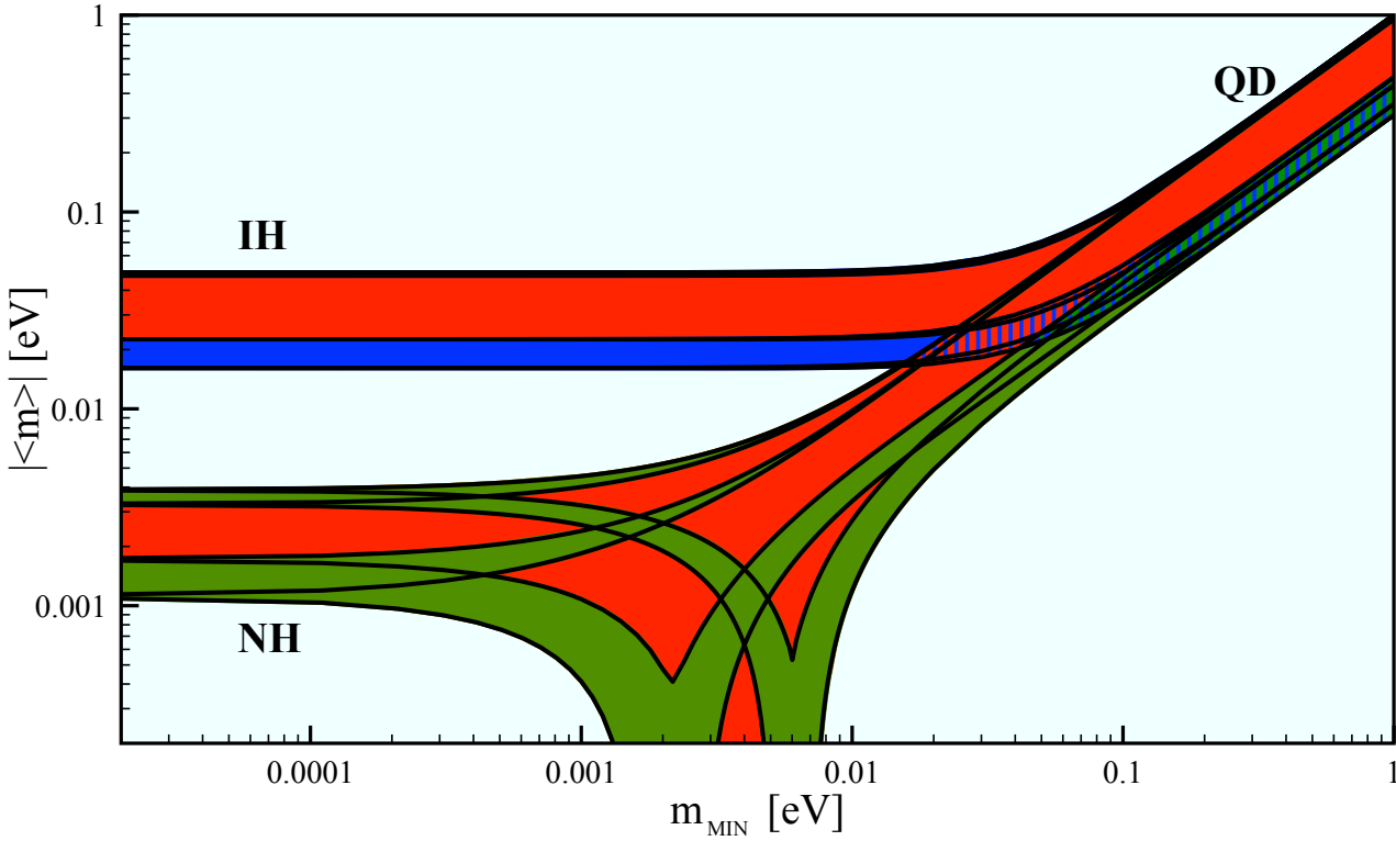
Figure 14.1: The effective Majorana mass |\langle m \rangle| (including a 2\sigma uncertainty), as a function of \min(m_j) . The figure is obtained using the best fit values and the 2\sigma ranges of allowed values of \Delta m_{21}^2 , \sin^2 \theta_{12} , and |\Delta m_{31}^2| \cong |\Delta m_{32}^2| from Ref. 60. The phases \alpha_{21,31} are varied in the interval [0, \pi] . The predictions for the NH, IH and QD spectra are indicated. The red regions correspond to at least one of the phases \alpha_{21,31} and (\alpha_{31} - \alpha_{21}) having a CP violating value, while the blue and green areas correspond to \alpha_{21,31} possessing CP conserving values. (Update by S. Pascoli of a figure from the one before the last article quoted in Ref. 91.)
