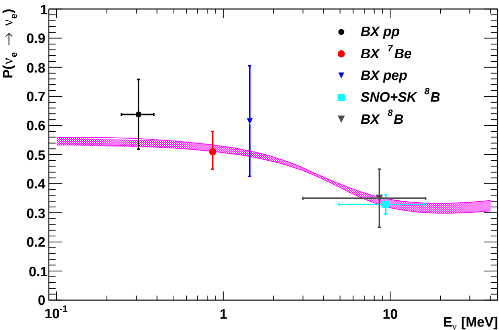
Figure 14.10: Electron neutrino survival probability as a function of neutrino energy according to the MSW-LMA model. The low-energy region ( < 1 MeV) of the curve is calculated for pp and ^7\text{Be} neutrinos, and the high-energy region for ^8\text{B} neutrinos, using the parameter values given in Ref. 52. The width of the curve reflects \pm 1\sigma uncertainties, determined by a Monte Carlo method sampling errors on parameters [52]. The points represent the Borexino pp, ^7\text{Be} , pep, and ^8\text{B} data and the SNO+SK ^8\text{B} data. This figure is provided by A. Ianni in the name of the BOREXINO Collaboration.
