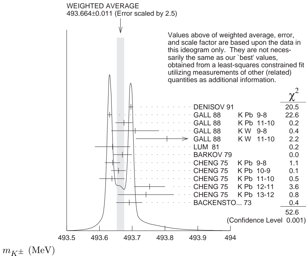
Figure 78.1: Ideogram of m_{K^\pm} mass measurements. GALL 88 and CHENG 75 measurements are shown separately for each transition they measured.
