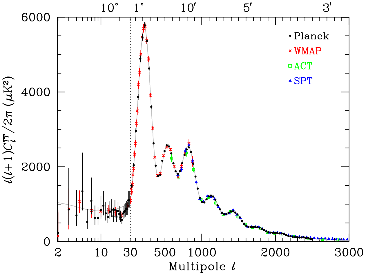
Figure 29.2: CMB temperature anisotropy band-power estimates from the Planck , WMAP , ACT , and SPT experiments. Note that the widths of the \ell -bands vary between experiments and have not been plotted. This figure represents only a selection of the most recent available experimental results, and some points with large error bars have been omitted. At the higher multipoles these band-powers involve subtraction of particular foreground models, and so proper analysis requires simultaneous fitting of CMB and foregrounds over multiple frequencies. The x -axis here is logarithmic for the lowest multipoles, to show the Sachs-Wolfe plateau, and linear for the other multipoles. The acoustic peaks and damping region are very clearly observed, with no need for a theoretical curve to guide the eye; however, the curve plotted is the best-fit Planck \Lambda CDM model.
