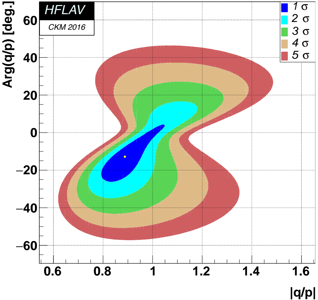
Figure 87.2: Two-dimensional 1\sigma - 5\sigma contours for (|q/p|, \text{Arg}(q/p)) from measurements of D^0 \rightarrow K^{(*)+}\ell\nu , h^+h^- , K^+\pi^- , K^+\pi^-\pi^0 , K^+\pi^-\pi^+\pi^- , K_S^0\pi^+\pi^- , K_S^0K^+K^- , and \pi^+\pi^-\pi^0 decays, and double-tagged branching fractions measured at the \psi(3770) resonance (from HFLAV [9]).
