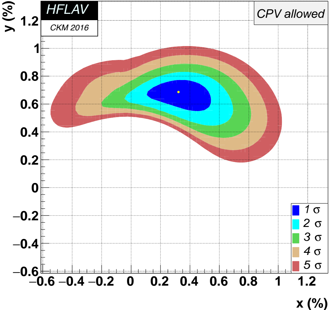
Figure 87.1: Two-dimensional 1\sigma - 5\sigma contours for (x, y) from measurements of D^0 \rightarrow K^{(*)+}\ell\nu , h^+h^- , K^+\pi^- , K^+\pi^-\pi^0 , K^+\pi^-\pi^+\pi^- , K_S^0\pi^+\pi^- , K_S^0K^+K^- , and \pi^+\pi^-\pi^0 decays, and double-tagged branching fractions measured at the \psi(3770) resonance (from HFLAV [9]).
