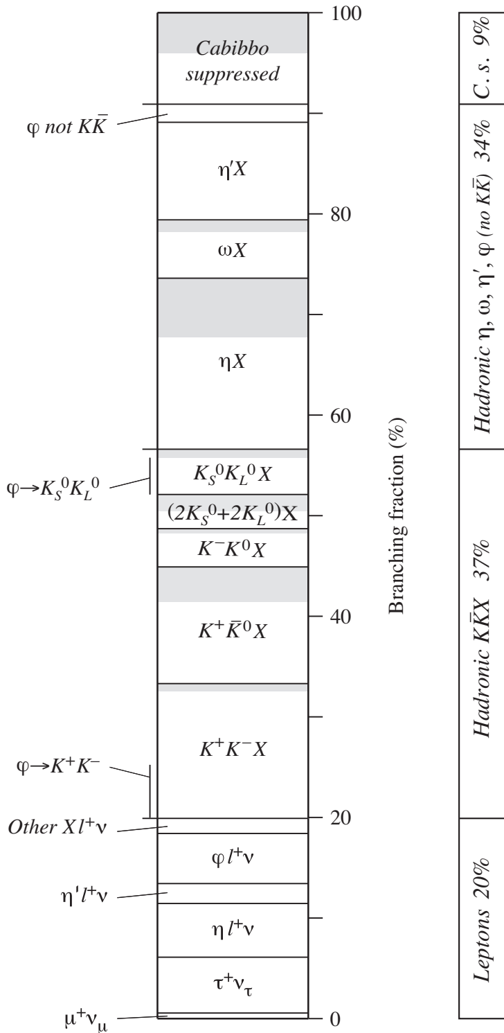
Figure 88.1: A partial breakdown of D_s^+ branching fractions. The hadronic bins in the left column show inclusive fractions. Shading within a bin shows how much of the inclusive fraction is not yet accounted for by adding up all the relevant exclusive fractions. The inclusive hadronic \phi fraction is spread over three bins, in proportion to its decay fractions into K^+K^- , K_S^0K_L^0 , and no- K\bar{K} modes.
