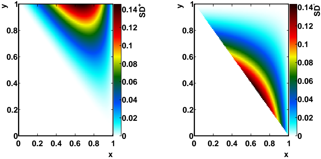
Figure 73.1: Components of the structure dependent terms of the decay width. Left: SD^+ , right: SD^-
