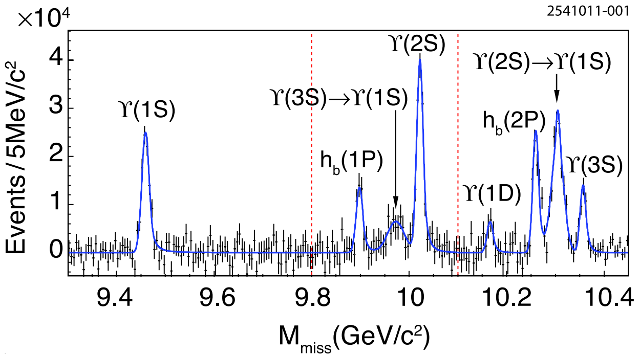
Figure 95.1: From Belle [44], the mass recoiling against \pi^+\pi^- pairs, M_{\text{miss}} , in e^+e^- collision data taken near the peak of the \Upsilon(10860) (points with error bars). The smooth combinatorial and K_S^0 \rightarrow \pi^+\pi^- background contributions have been subtracted. The fit to the various labeled signal contributions is overlaid (curve). Adapted from [44] with kind permission, copyright (2011) The American Physical Society.
