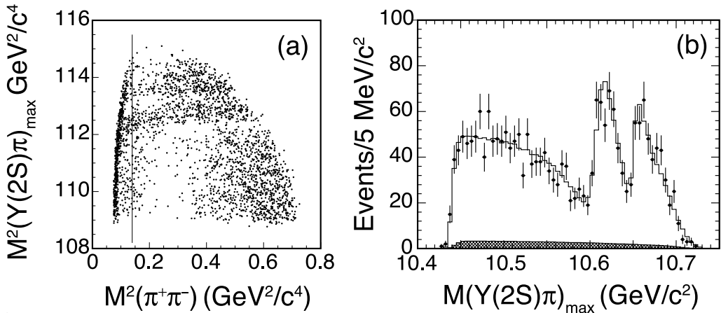
Figure 95.4: From Belle [80] e^+e^- collision data taken near the peak of the \Upsilon(10860) for events with a \pi^+\pi^- -missing mass consistent with an \Upsilon(2S) \rightarrow \mu^+\mu^- , (a) the maximum of the two possible single \pi^\pm -missing-mass-squared combinations vs. the \pi^+\pi^- -mass-squared; and (b) projection of the maximum of the two possible single \pi^\pm -missing-mass combinations ( points with error bars ) overlaid with a fit ( curve ). Events to the left of the vertical line in (a) are excluded from amplitude analysis. The hatched histogram in (b) corresponds to the combinatorial background. The two horizontal stripes in (a) and two peaks in (b) correspond to the two Z_b states. Adapted from [80] with kind permission, copyright (2011) The American Physical Society.
