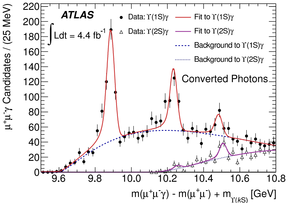
Figure 95.2: From ATLAS [48] pp collision data (points with error bars) taken at \sqrt{s} = 7 TeV, the effective mass of \chi_{bJ}(1P, 2P, 3P) \rightarrow \gamma\Upsilon(1S, 2S) candidates in which \Upsilon(1S, 2S) \rightarrow \mu^+\mu^- and the photon is reconstructed as an e^+e^- conversion in the tracking system. Fits (smooth curves) show significant signals for each triplet ( J -merged) on top of a smooth background. From [48] with kind permission, copyright (2012) The American Physical Society.
