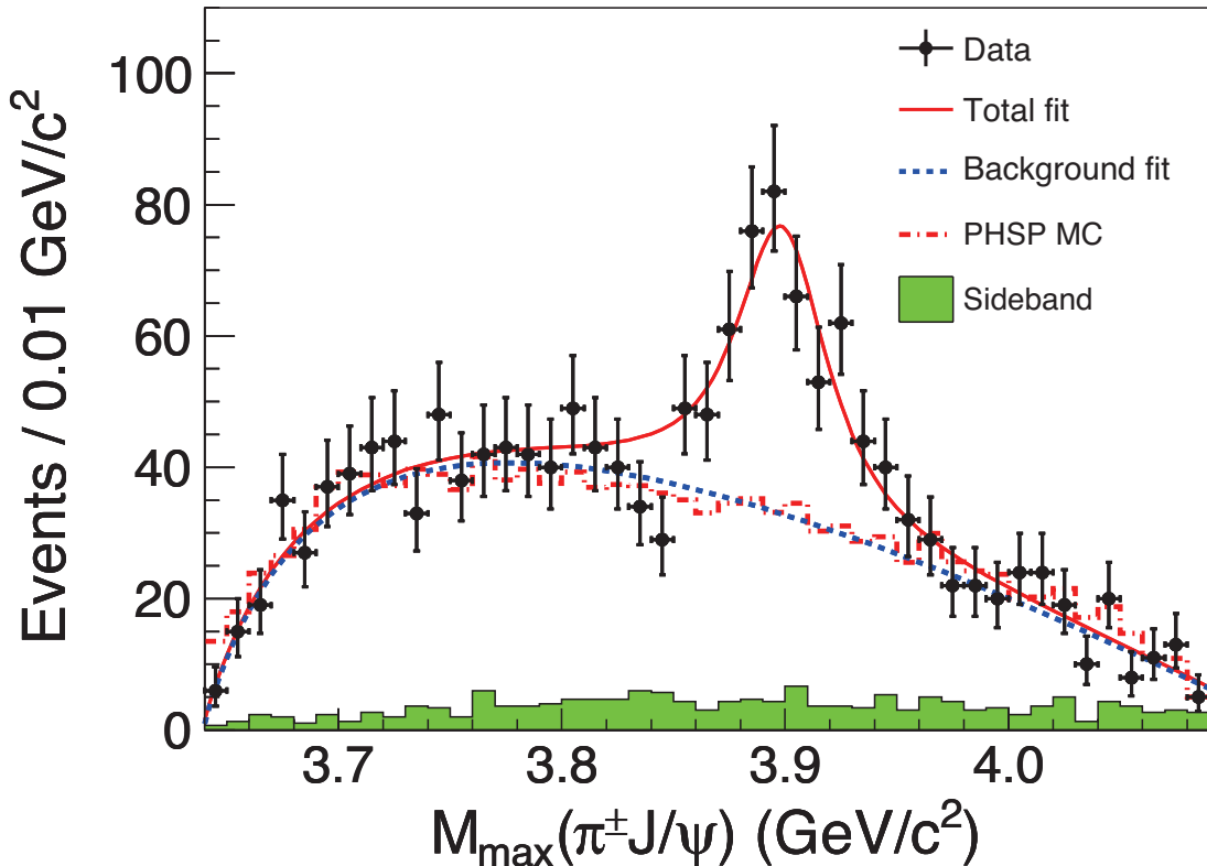
Figure 95.3: J/\psi\pi invariant mass distributions from BES-III [70] e^+e^- collision data taken near the peak of the Y(4260) . Adapted from [70] with kind permission, copyright (2013) The American Physical Society.
