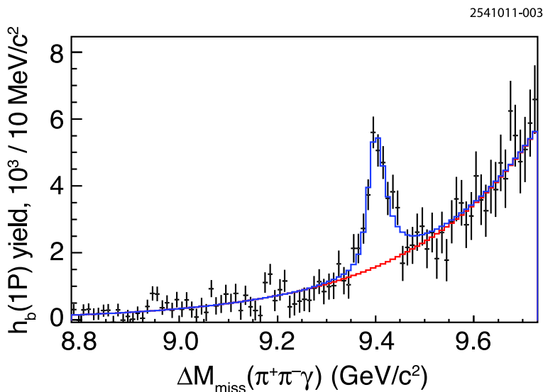
Figure 95.5: From Belle [43] e^+e^- collision data taken near the peak of the \Upsilon(10860) , the h_b(1P) event yield vs. the mass recoiling against the \pi^+\pi^-\gamma (corrected for misreconstructed \pi^+\pi^- ), where the h_b(1P) yield is obtained by fitting the mass recoiling against the \pi^+\pi^- ( points with error bars ). The fit results ( solid histograms ) for signal plus background and background alone are superimposed.
