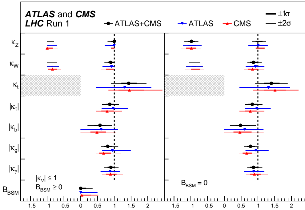
Figure 11.12: ATLAS-CMS combined measurements of coupling modifiers.
