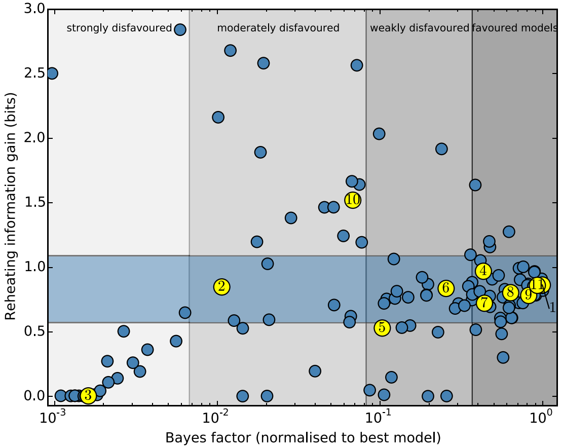
Figure 23.3: The Bayes factors calculated in [84] for a large sample of inflationary models. Those highlighted in yellow are featured in this review, according to the numbers listed in the text.
