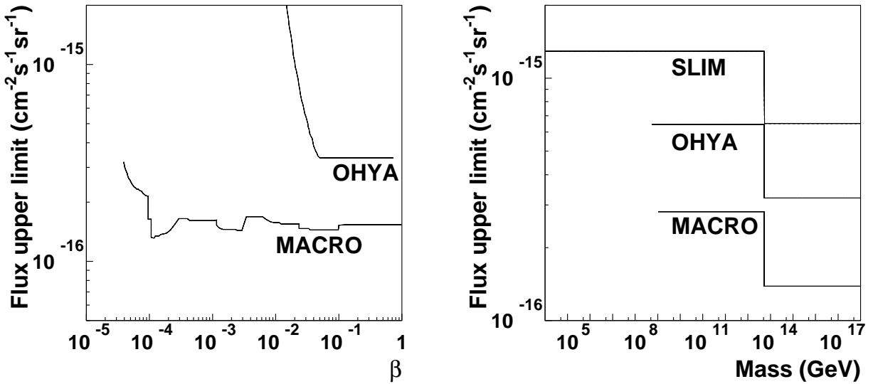
Figure 111.1: Upper flux limits for (a) GUT monopoles as a function of \beta (b) Monopoles as a function of mass for \beta > 0.05 .
