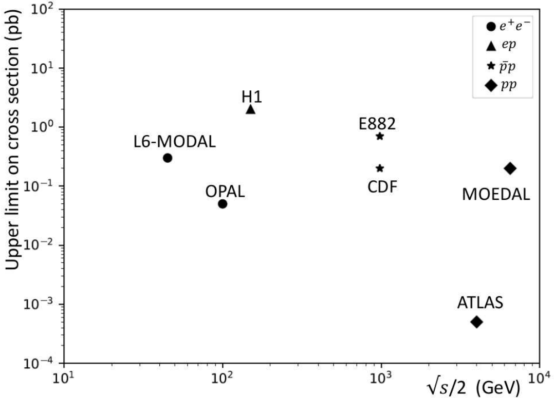
Figure 111.2: Upper limits on the production cross sections of monopoles from various collider-based experiments.
