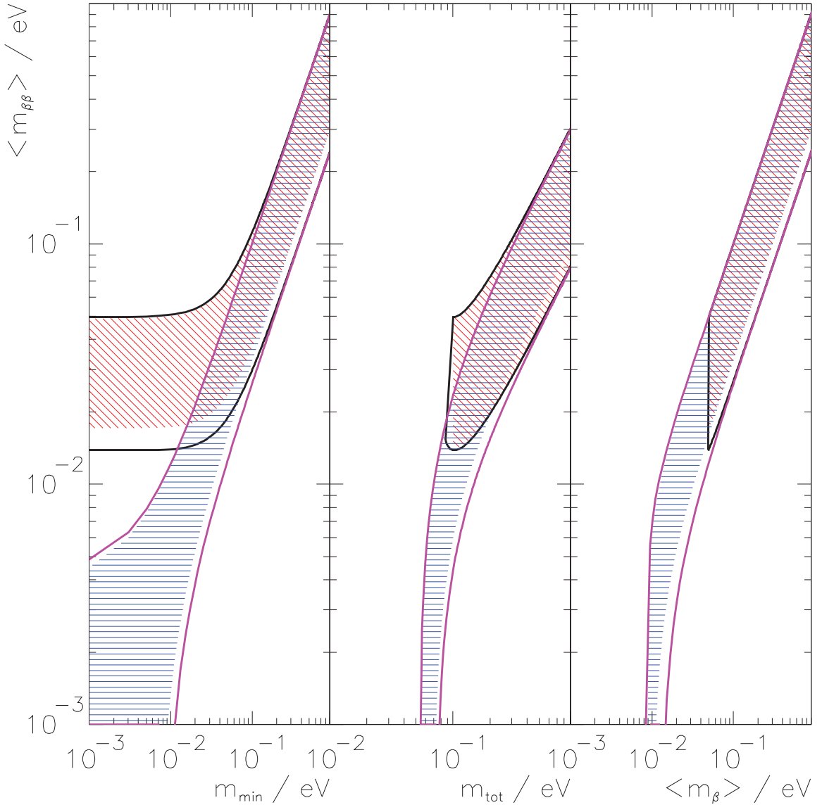
Figure 69.1: The left panel shows the dependence of \langle m_{\beta\beta} \rangle on the absolute mass of the lightest neutrino m_{\min} . The middle panel shows \langle m_{\beta\beta} \rangle as a function of the summed neutrino mass m_{\text{tot}} , while the right panel depicts \langle m_{\beta\beta} \rangle as a function of the mass \langle m_{\beta} \rangle . In all panels the width of the hatched areas is due to the unknown Majorana phases and thus irreducible. The allowed areas given by the solid lines are obtained by taking into account the errors of the oscillation parameters (at 90% confidence level [1]). The two sets of solid lines correspond to the normal (blue) and inverted (red) hierarchies. These sets merge into each other for \langle m_{\beta\beta} \rangle \geq 0.1 eV, which corresponds to the degenerate mass pattern.
