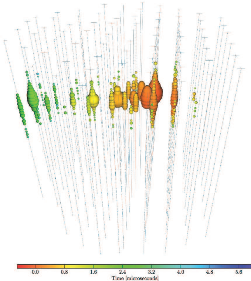
Figure 36.8: Event display of one of the starting-track events from [53]. The deposited energy is 70 TeV, the colour code indicates the signal timing (red: early; green: late).
