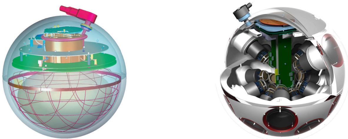
Figure 36.6: Schematic views of the digital OMs of IceCube (left) and KM3NeT (right).
