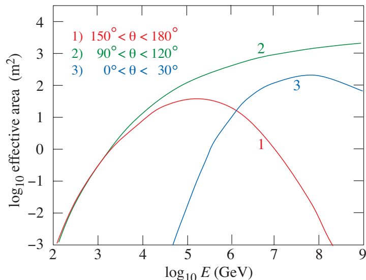
Figure 36.5: Effective \bar{\nu}_\mu area for IceCube as an example of a cubic-kilometre NT, as a function of neutrino energy for three intervals of the zenith angle \theta . The values shown here correspond to a specific event selection for point source searches.
