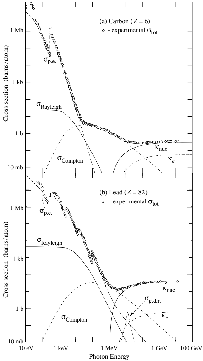
Figure 34.15: Photon total cross sections as a function of energy in carbon and lead, showing the contributions of different processes [50]:
