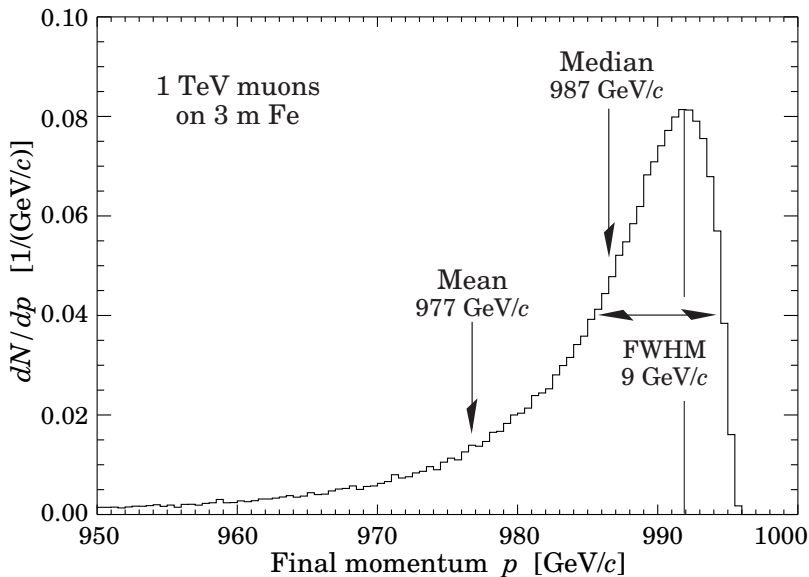
Figure 34.25: The momentum distribution of 1 TeV/c muons after traversing 3 m of iron as calculated with the MARS15 Monte Carlo code [71] by S.I. Striganov [5].
