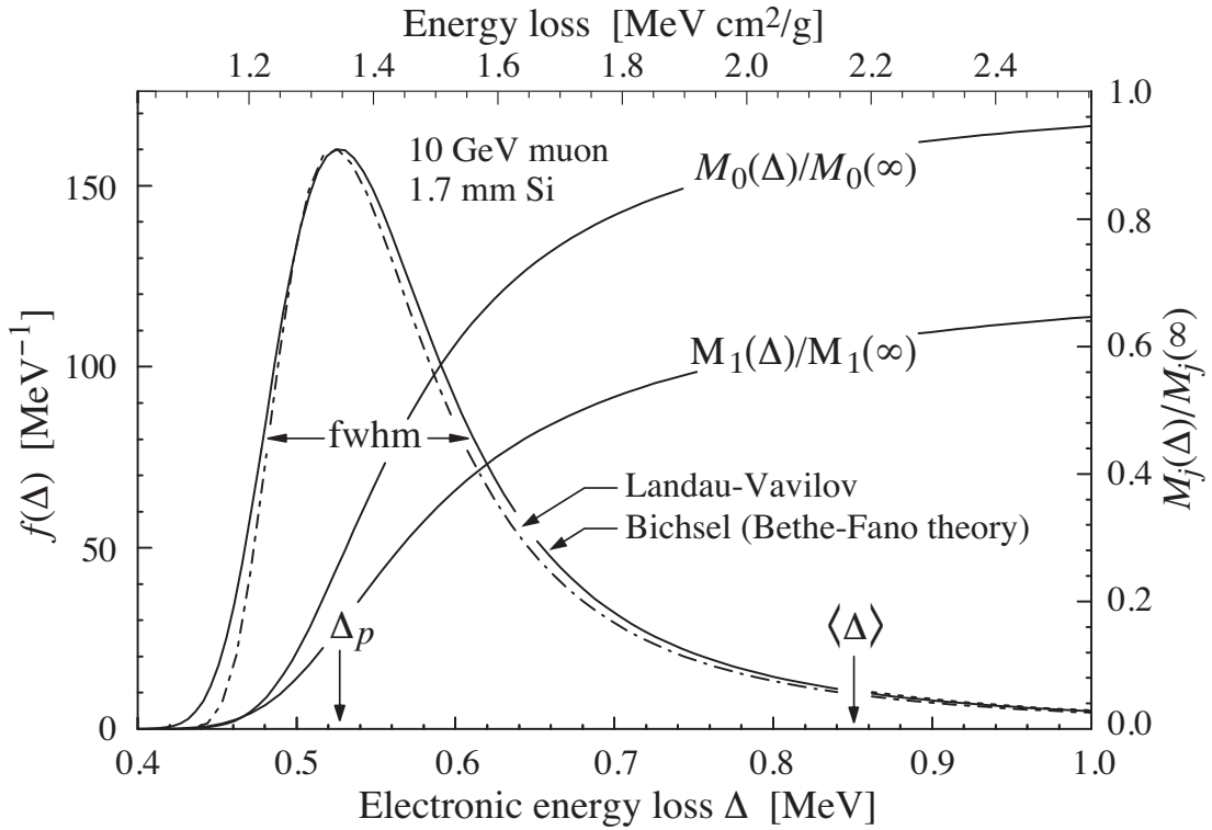
Figure 34.7: Electronic energy deposit distribution for a 10 GeV muon traversing 1.7 mm of silicon, the stopping power equivalent of about 0.3 cm of PVT-based scintillator [1,13,28]. The Landau-Vavilov function (dot-dashed) uses a Rutherford cross section without atomic binding corrections but with a kinetic energy transfer limit of W_{\max} . The solid curve was calculated using Bethe-Fano theory. M_0(\Delta) and M_1(\Delta) are the cumulative 0th moment (mean number of collisions) and 1st moment (mean energy loss) in crossing the silicon. (See Sec. 34.2.1. The fwhm of the Landau-Vavilov function is about 4\xi for detectors of moderate thickness. \Delta_p is the most probable energy loss, and \langle\Delta\rangle divided by the thickness is the Bethe \langle dE/dx \rangle ).
