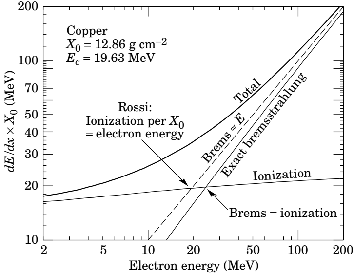
Figure 34.13: Two definitions of the critical energy E_c .
