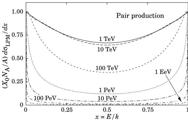
Figure 34.18: The normalized pair production cross section d\sigma_{LPM}/dy , versus fractional electron energy x = E/k .
