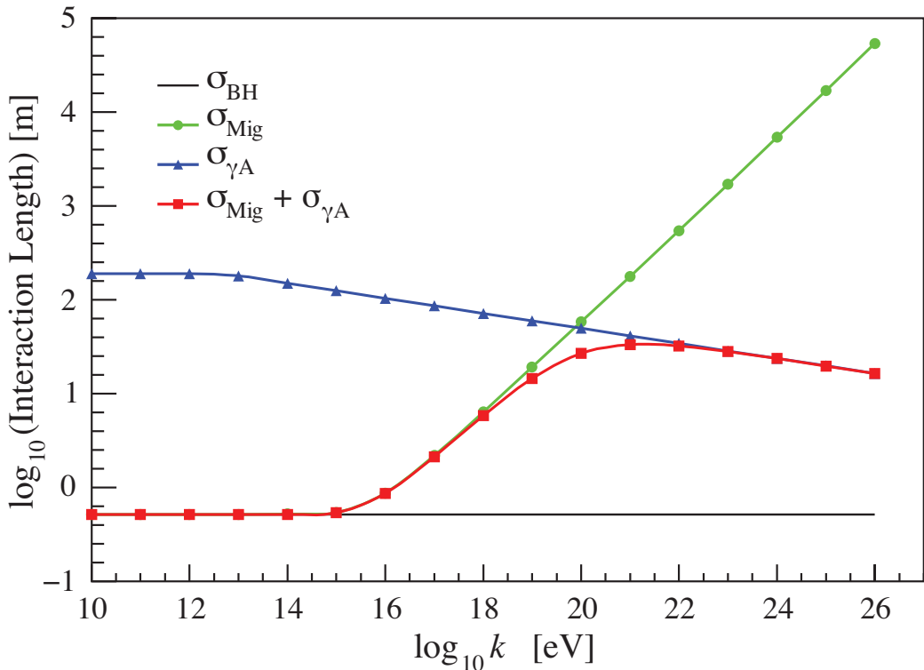
Figure 34.19: Interaction length for a photon in ice as a function of photon energy for the Bethe-Heitler (BH), LPM (Mig) and photonuclear ( \gamma A ) cross sections [55]. The Bethe-Heitler interaction length is 9X_0/7 , and X_0 is 0.393 m in ice.
