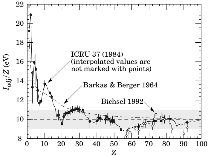
Figure 34.5: Mean excitation energies (divided by Z ) as adopted by the ICRU [11]. Those based on experimental measurements are shown by symbols with error flags; the interpolated values are simply joined. The grey point is for liquid \text{H}_2 ; the black point at 19.2 eV is for \text{H}_2 gas. The open circles show more recent determinations by Bichsel [13]. The dash-dotted curve is from the approximate formula of Barkas [14] used in early editions of this Review .
