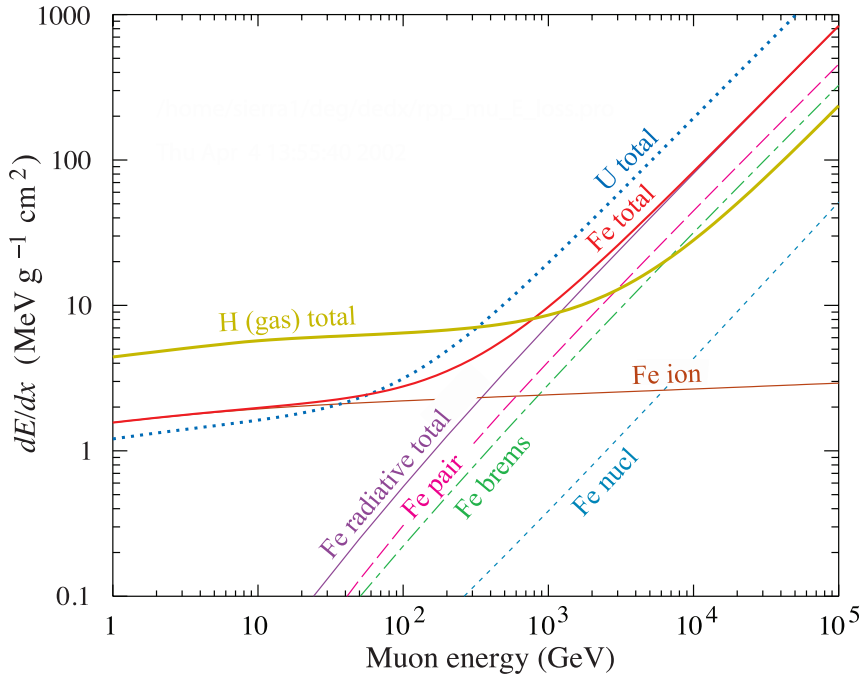
Figure 34.23: The average energy loss of a muon in hydrogen, iron, and uranium as a function of muon energy. Contributions to dE/dx in iron from ionization and the processes shown in Fig. 34.22 are also shown.
