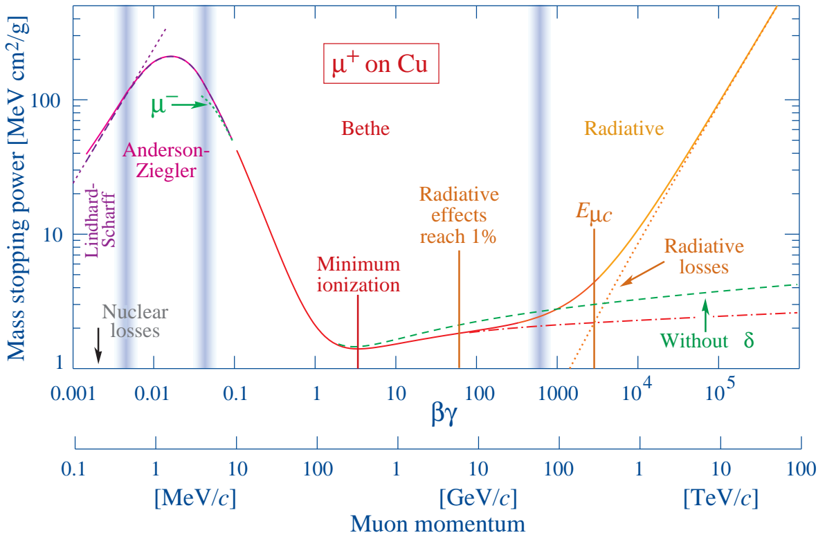
Fig. 34.1: Mass stopping power ( = \langle -dE/dx \rangle ) for positive muons in copper as a function of \beta\gamma = p/Mc over nine orders of magnitude in momentum (12 orders of magnitude in kinetic energy). Solid curves indicate the total stopping power. Data below the break at \beta\gamma \approx 0.1 are taken from ICRU 49 [4], and data at higher energies are from Ref. 5. Vertical bands indicate boundaries between different approximations discussed in the text. The short dotted lines labeled “ \mu^- ” illustrate the “Barkas effect,” the dependence of stopping power on projectile charge at very low energies [6]. dE/dx in the radiative region is not simply a function of \beta .
