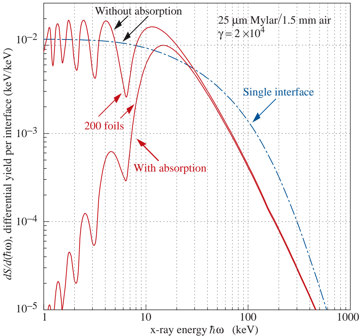
Figure 34.27: X-ray photon energy spectra for a radiator consisting of 200 25\ \mu\text{m} thick foils of Mylar with 1.5 mm spacing in air (solid lines) and for a single surface (dashed line). Curves are shown with and without absorption. Adapted from Ref. 87.
