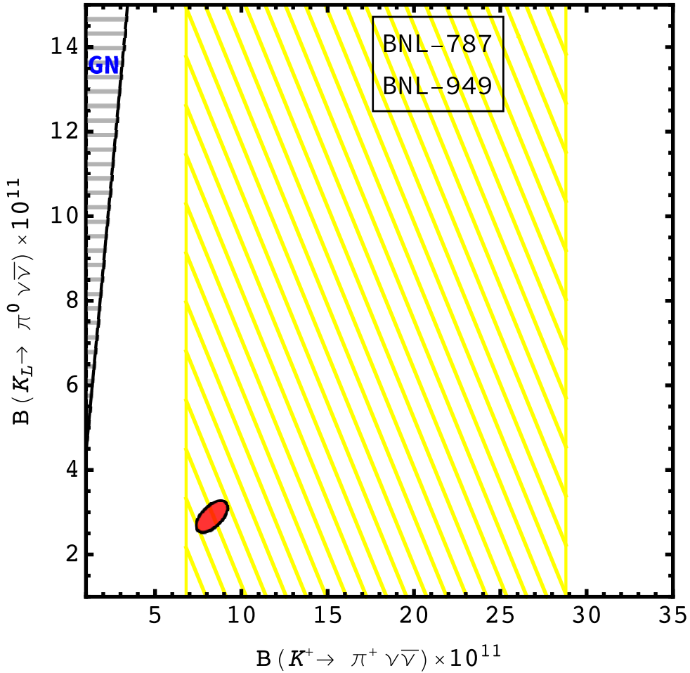
Figure 79.2: Summary of current situation for the golden modes K \rightarrow \pi \nu \bar{\nu} . The red and yellow regions correspond to the 90% CL SM prediction with input from CKMfitter and to the BNL measurement respectively. The black dashed region shows the GN exclusion.
