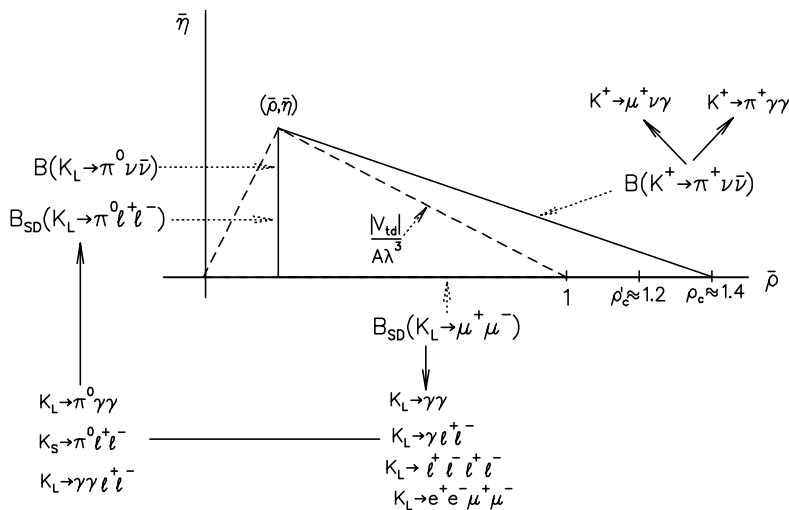
Figure 79.1: Role of rare kaon decays in determining the unitarity triangle. The solid arrows point to auxiliary modes needed to interpret the main results, or potential backgrounds to them.
