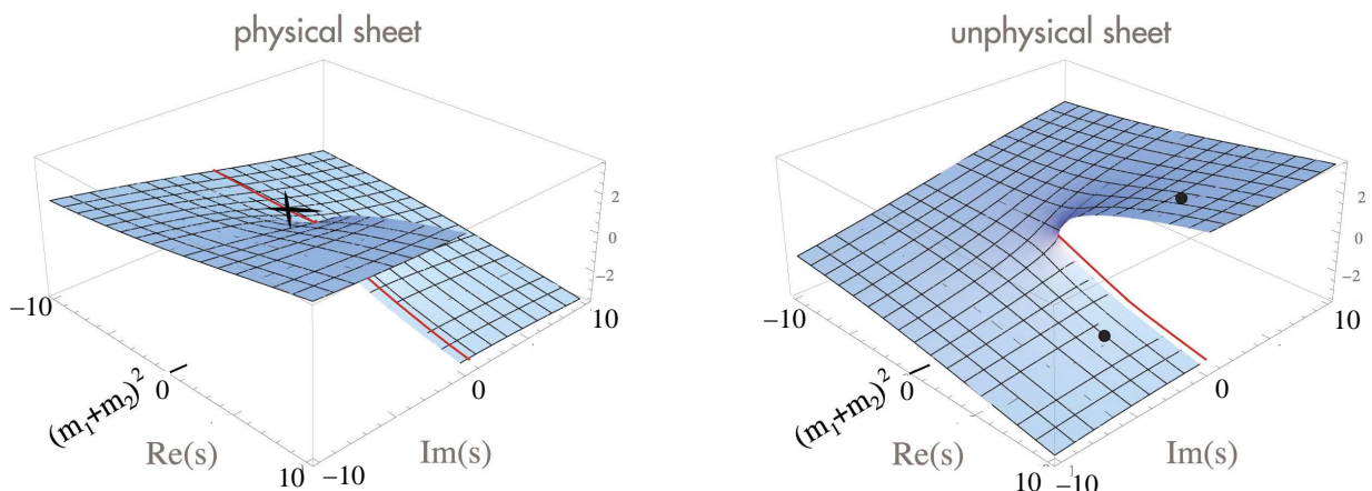
Figure 49.1: Sketch of the imaginary part of a typical single-channel amplitude in the complex s -plane. The solid dots indicate allowed positions for resonance poles, the cross for a bound state. The solid line is the physical axis (shifted by i\epsilon into the physical sheet). The two sheets are connected smoothly along their discontinuities.
