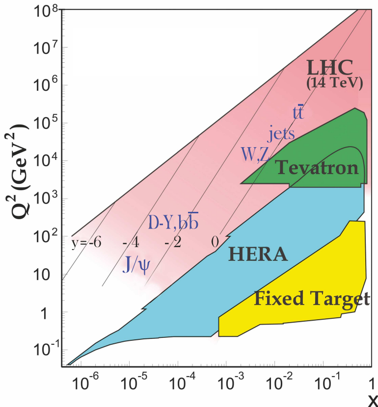
Figure 19.4: Kinematic domains in x and Q^2 probed by fixed-target and collider experiments. Some of the final states accessible at the LHC are indicated in the appropriate regions, where y is the rapidity. The incoming partons have x_{1,2} = (M/14 \text{ TeV})e^{\pm y} with Q = M where M is the mass of the state shown in blue in the figure. For example, exclusive J/\psi and \Upsilon production at high |y| at the LHC may probe the gluon PDF down to x \sim 10^{-5} .
