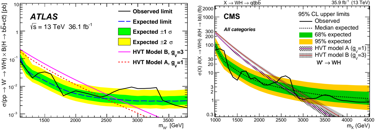
Figure 58.2: Upper limits at 95% CL on W' production cross section times branching fraction into a W and a SM Higgs boson, from [41] (left) and [44] (right).
