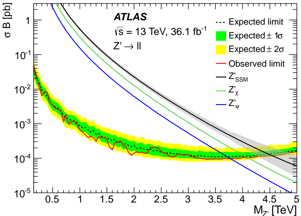
Figure 59.1: Upper limit on \sigma(pp \rightarrow Z'X \rightarrow \ell^+\ell^-X) with \ell = e or \mu as a function of M_{Z'} [24], assuming equal couplings for electrons and muons. The lines labelled by Z'_\psi and Z'_\chi are theoretical predictions for the U(1)_{10+x5} models in Table 59.1 with x = -3 and x = +1 , respectively, for g_z fixed by an E_6 unification condition. The Z'_{\text{SSM}} line corresponds to Z' couplings equal to those of the Z boson.
