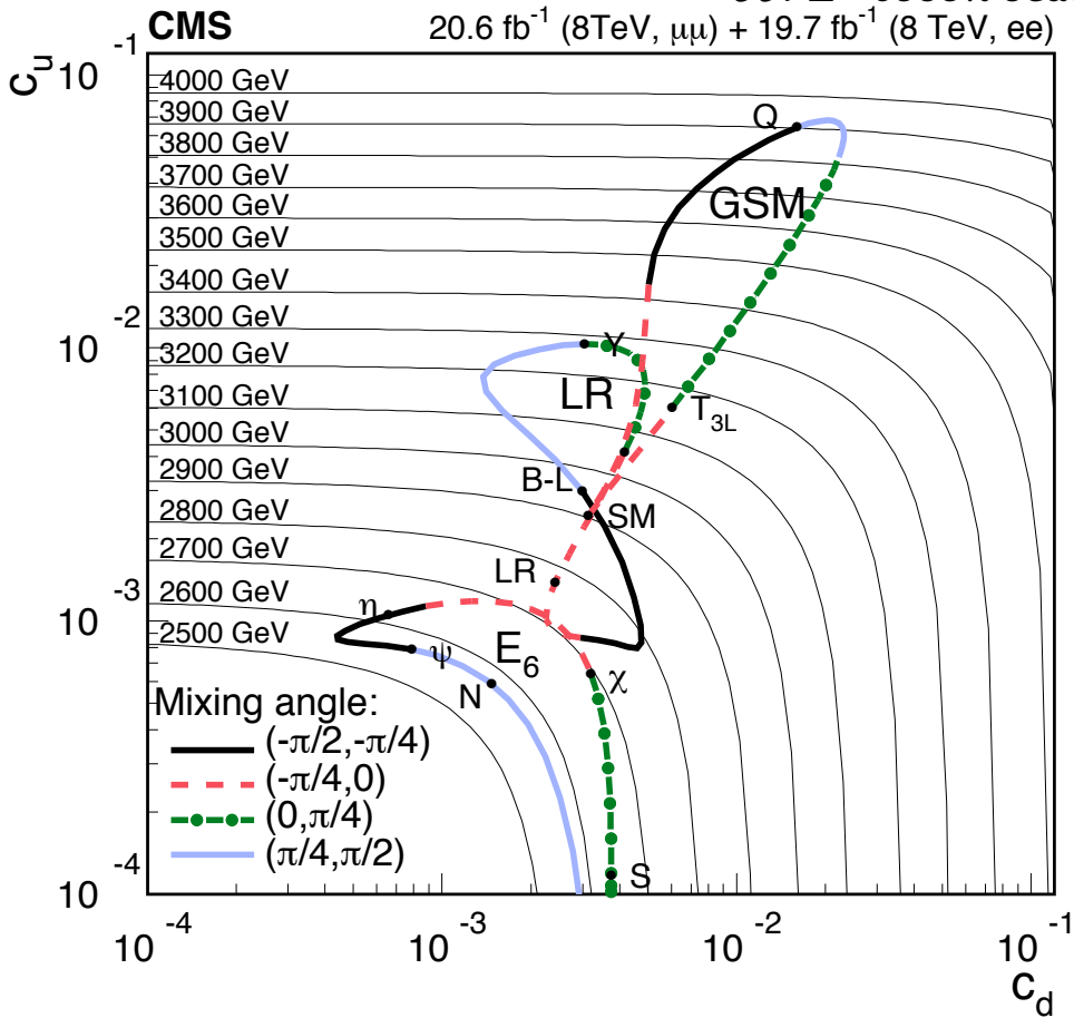
Figure 59.2: Upper limits in the c_u^\ell - c_d^\ell plane ( \ell = e or \mu ), set by CMS [23], are shown as thin lines for certain M_{Z'} values. For specific sets of charges (labelled by E_6 , GSM and LR, and described in [7]) parametrized by a mixing angle, the lower mass limit is given by the intersection of thick and thin lines. The black dots with smaller labels represent particular models.
