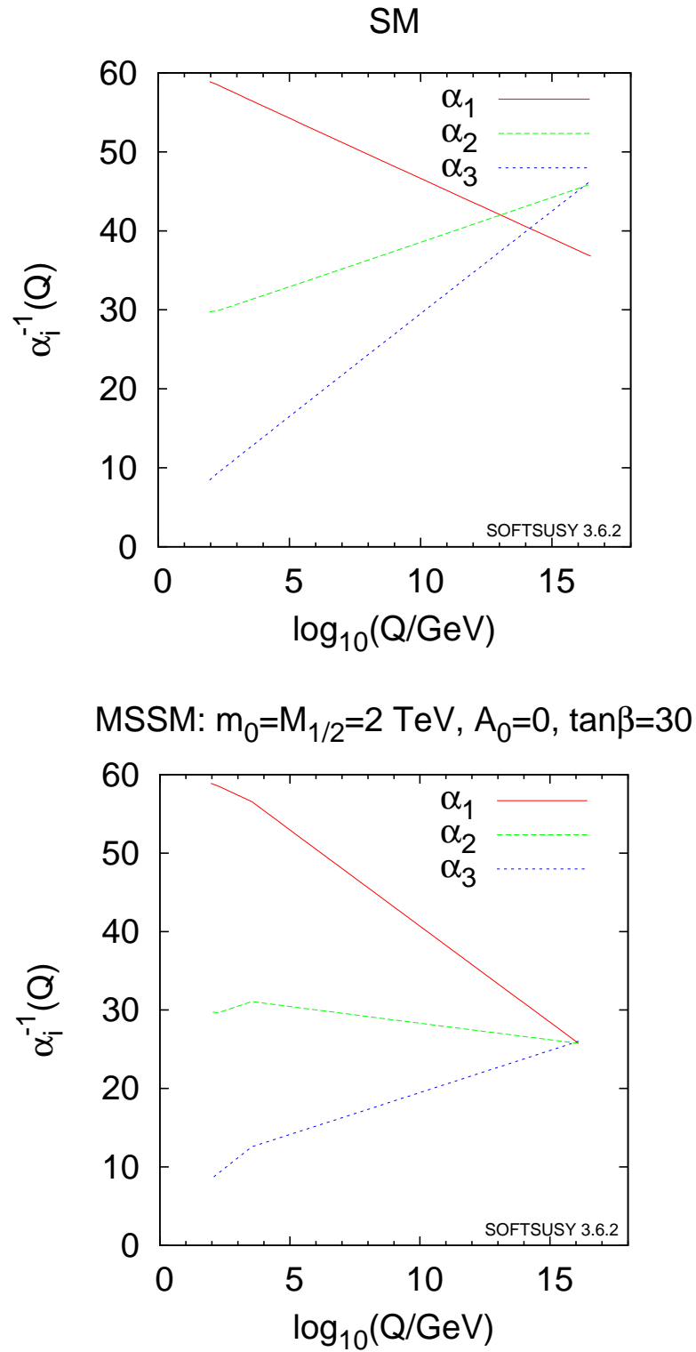
Figure 16.1: Running couplings in SM and MSSM using two-loop RG evolution. The SUSY threshold at 2 TeV is clearly visible on the r.h. side. (We thank Ben Allanach for providing the plots created using SOFTSUSY [61].)
