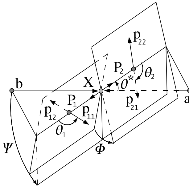
Figure 92.1: Definition of the production and helicity angles in the sequential process ab \rightarrow X \rightarrow P_1 P_2 \rightarrow (p_{11} p_{12})(p_{21} p_{22}) . The three helicity angles include \theta_1 and \theta_2 , defined in the rest frame of the two daughters P_1 and P_2 , and \Phi , defined in the X frame as the angle between the two decay planes. The two production angles \theta^* and \Psi are defined in the X frame, where \Psi is the angle between the production plane and the average of the two decay planes.
