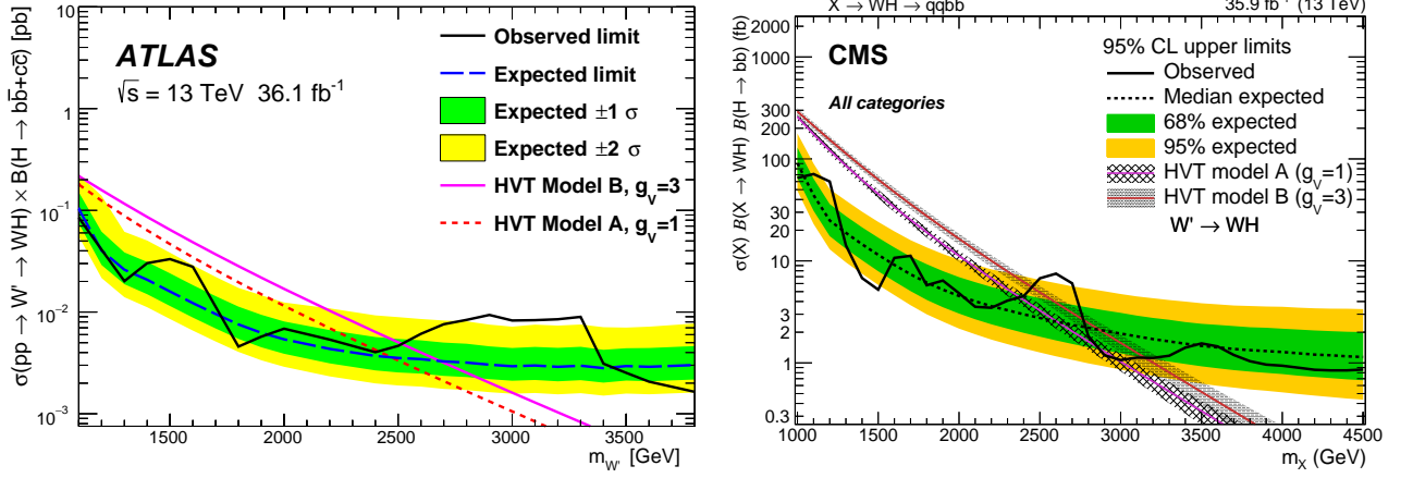
Figure 58.2: Upper limits at 95% CL on W' production cross section times branching fraction into a W and a SM Higgs boson, from [41] (left) and [44] (right).
