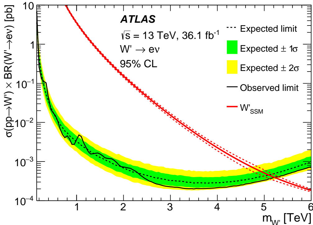
Figure 58.1: Upper limit on \sigma(pp \rightarrow W'X) B(W' \rightarrow e\nu) from ATLAS [16], at 95% CL. The red line shows the theoretical prediction in the Sequential SM.
