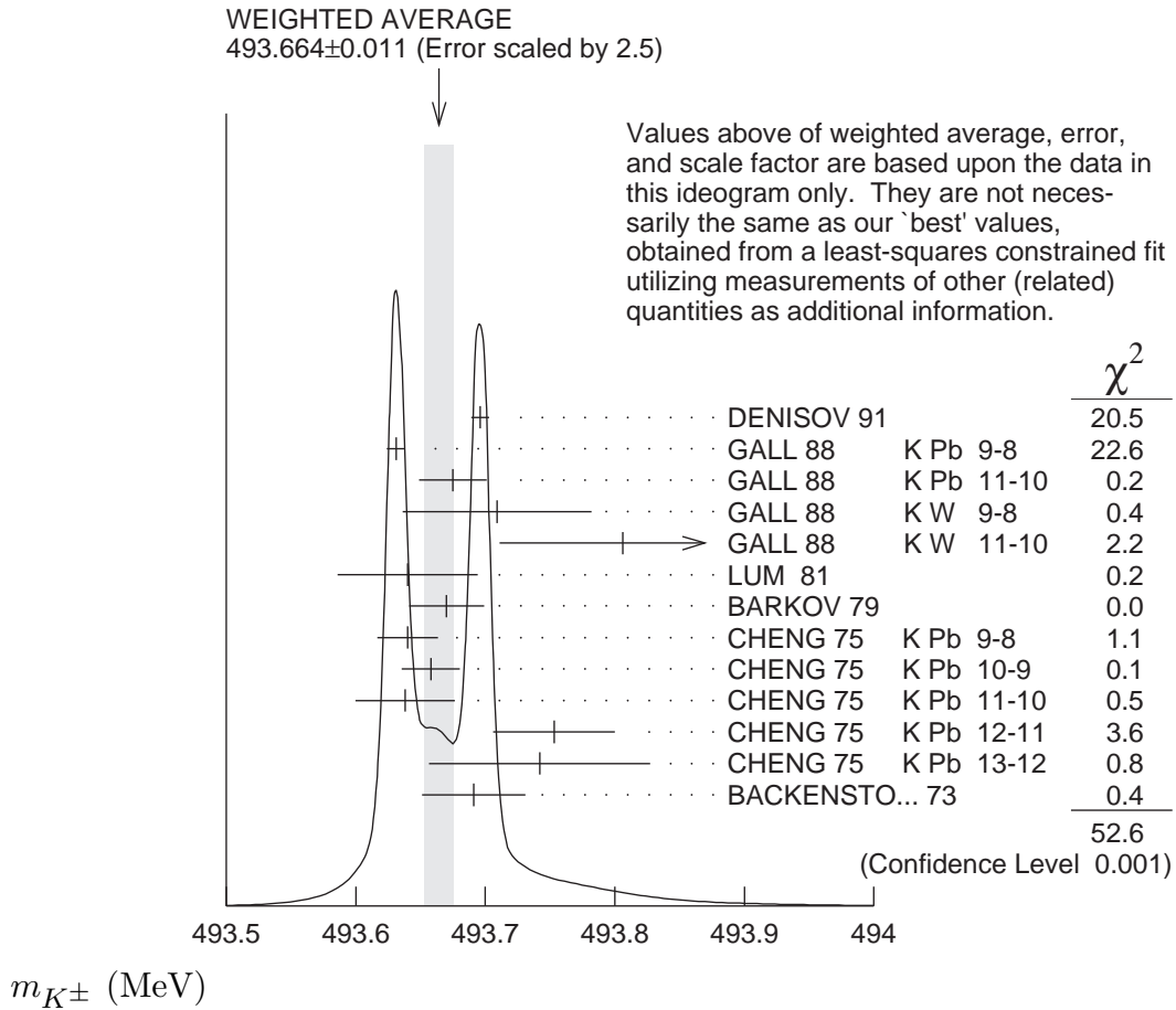
Figure 73.1: Ideogram of m_{K^\pm} mass measurements. GALL 88 and CHENG 75 measurements are shown separately for each transition they measured.
