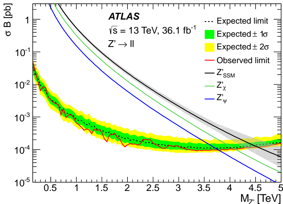
Figure 108.1: Upper limit on \sigma(pp \rightarrow Z' X \rightarrow \ell^+ \ell^- X) with \ell = e or \mu as a function of M_{Z'} [24], assuming equal couplings for electrons and muons. The lines labelled by Z'_\psi and Z'_\chi are theoretical predictions for the U(1)_{10+x5} models in Table 108.1 with x = -3 and x = +1 , respectively, for g_z fixed by an E_6 unification condition. The Z'_{\text{SSM}} line corresponds to Z' couplings equal to those of the Z boson.
