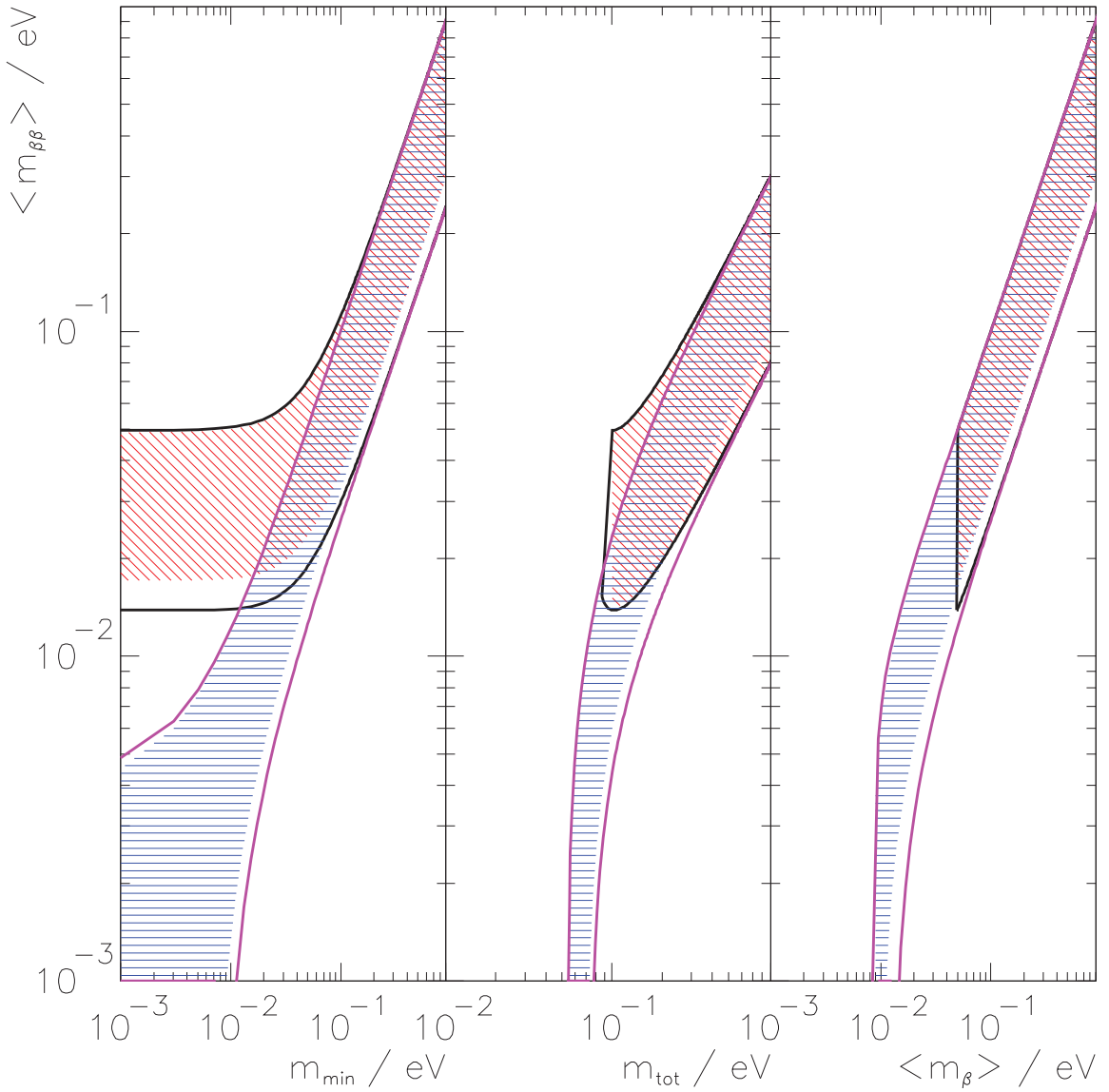
Figure 62.1: The left panel shows the dependence of \langle m_{\beta\beta} \rangle on the absolute mass of the lightest neutrino m_{\min} . The middle panel shows \langle m_{\beta\beta} \rangle as a function of the summed neutrino mass m_{\text{tot}} , while the right panel depicts \langle m_{\beta\beta} \rangle as a function of the mass \langle m_{\beta} \rangle . In all panels the width of the hatched areas is due to the unknown Majorana phases and thus irreducible. The allowed areas given by the solid lines are obtained by taking into account the errors of the oscillation parameters (at 90% confidence level [1]). The two sets of solid lines correspond to the normal (blue) and inverted (red) hierarchies. These sets merge into each other for \langle m_{\beta\beta} \rangle \geq 0.1 eV, which corresponds to the degenerate mass pattern.
