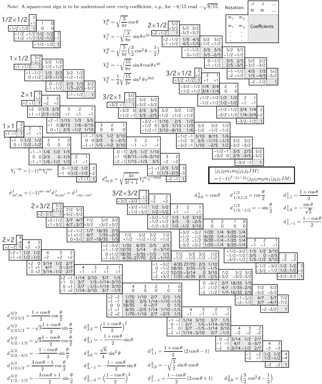
Figure 46.1: The sign convention is that of Wigner ( Group Theory , Academic Press, New York, 1959), also used by Condon and Shortley ( The Theory of Atomic Spectra , Cambridge Univ. Press, New York, 1953), Rose ( Elementary Theory of Angular Momentum , Wiley, New York, 1957), and Cohen ( Tables of the Clebsch-Gordan Coefficients , North American Rockwell Science Center, Thousand Oaks, Calif., 1974).
