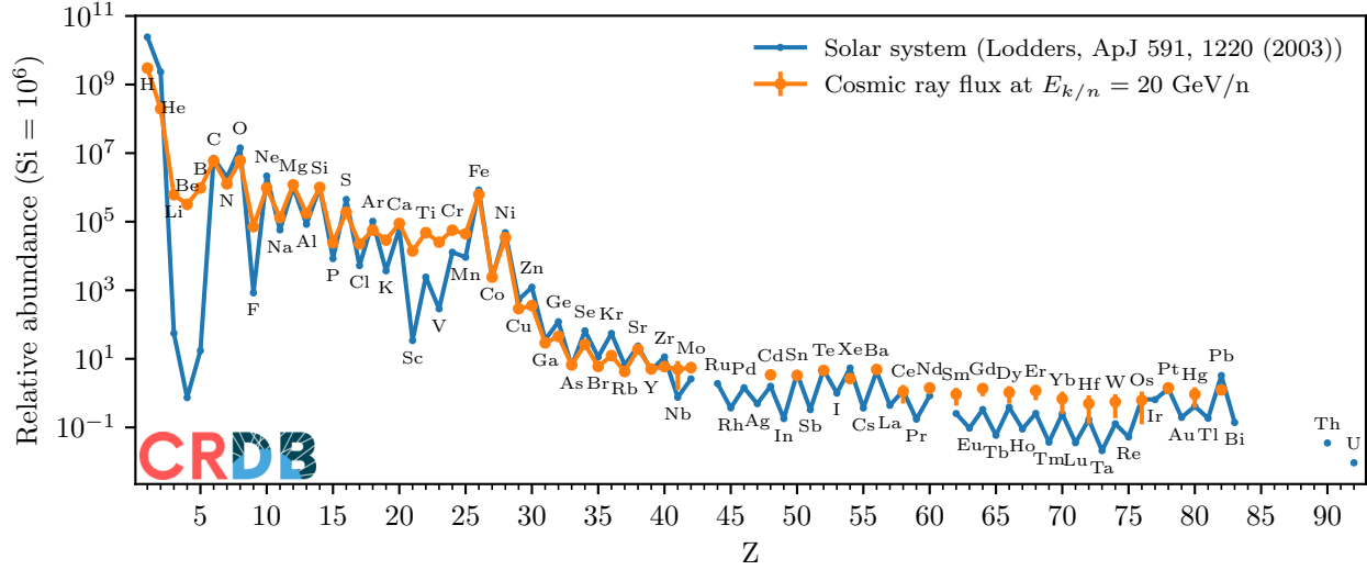
Figure 30.2: CR abundances compared with solar system ones [58]. Modified from [35].
