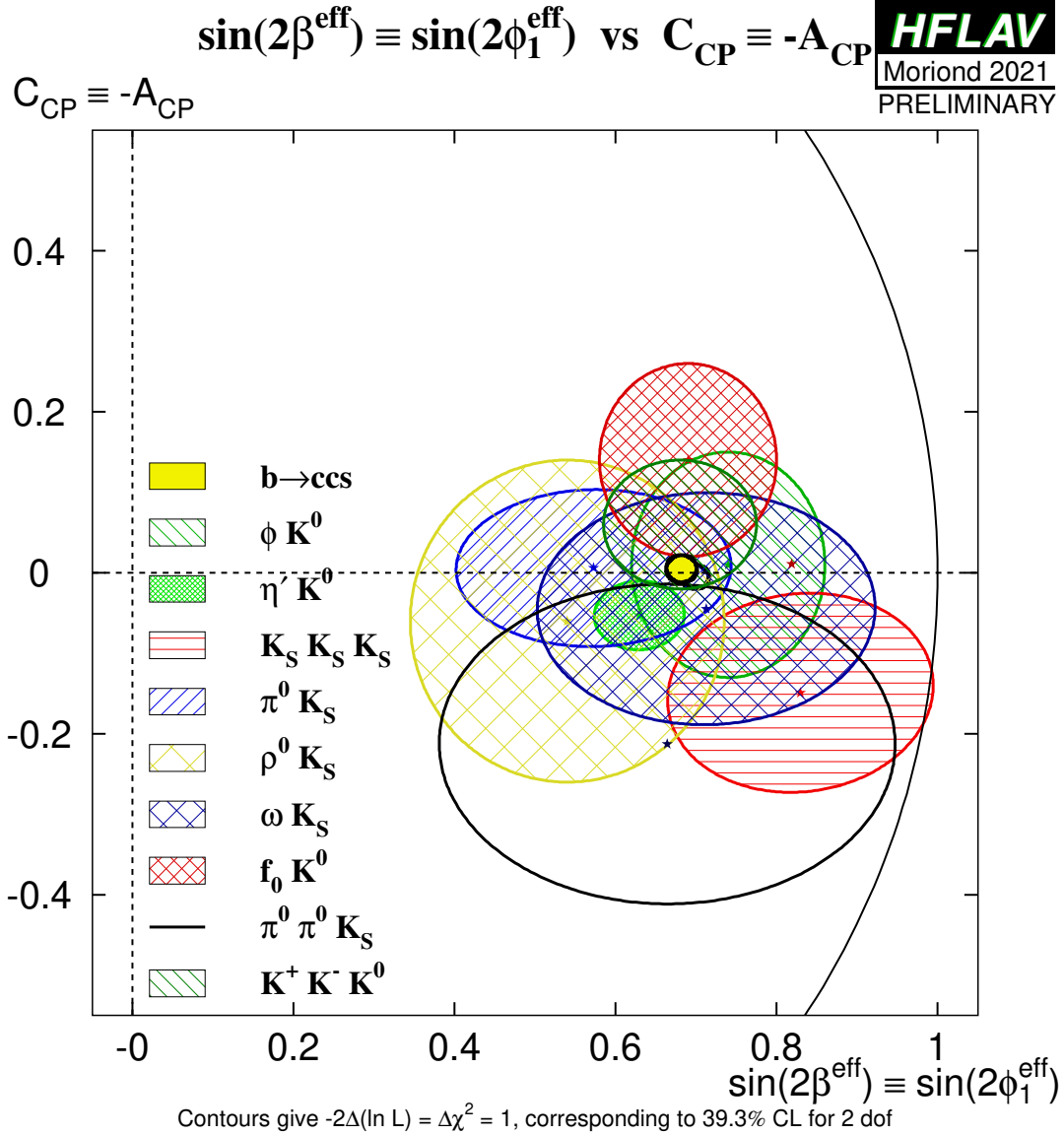
Figure 13.3: Summary of the results [62] of time-dependent analyses of b \rightarrow q\bar{q}s decays, which are potentially sensitive to new physics.
