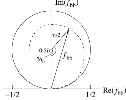
Figure 50.5: Argand plot showing a trajectory of the diagonal element of a partial-wave amplitude, f_{bb} , as a function of energy in the complex plane. As the energy increases the amplitude follows the line counter clockwise. The amplitude leaves the unitary circle (solid line) as soon as inelasticity sets in, \eta < 1 (dashed line).
