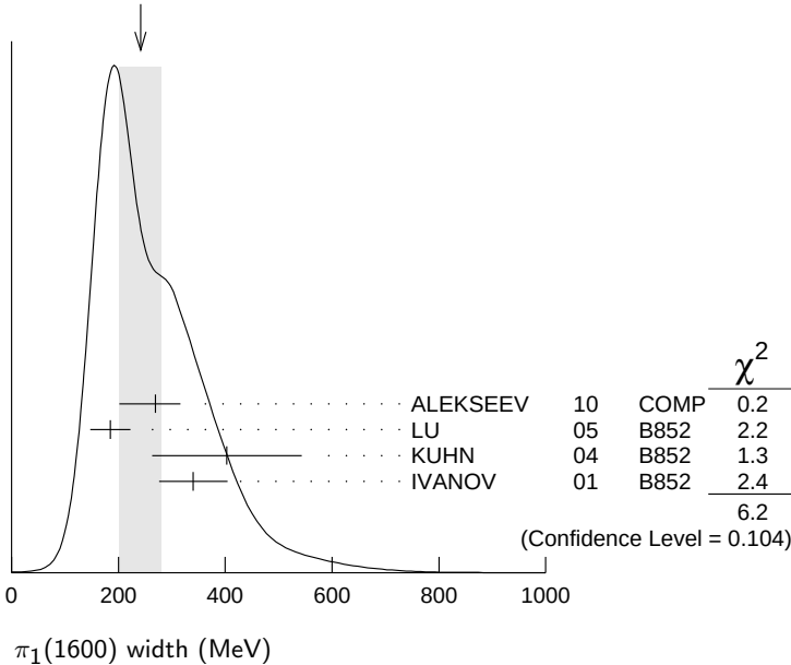
WEIGHTED AVERAGE 241±40 (Error scaled by 1.4)
