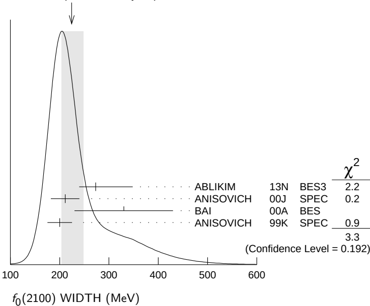
WEIGHTED AVERAGE 224+23-21 (Error scaled by 1.3)
