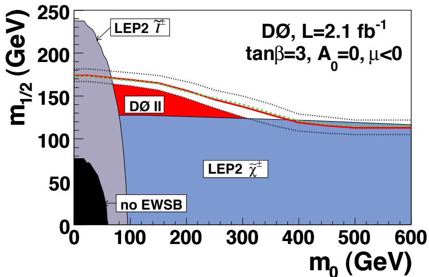
Figure 4: Region in the (m_0, m_{1/2}) plane excluded by the search for squarks and gluinos by DØ and by the searches for sleptons and charginos by the LEP experiments. The band at the edge of the excluded region represents the uncertainty associated with the scale and PDF choice, with the red curve corresponding to the nominal choice.
