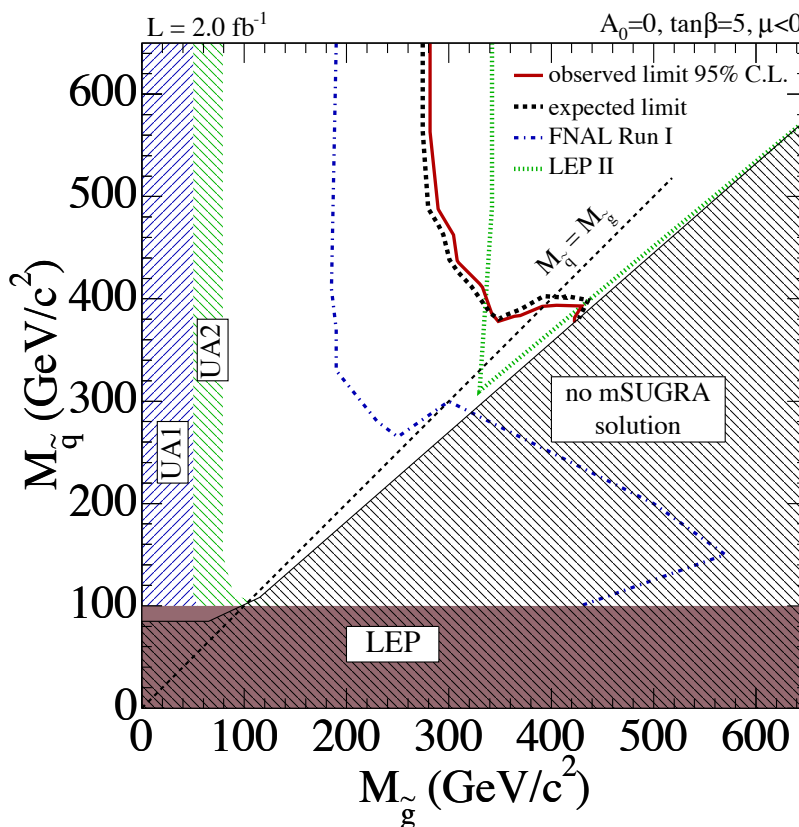
Figure 3: Region in the (m_{\tilde{g}}, m_{\tilde{q}}) plane excluded by CDF Run II and by earlier experiments. Color version at end of book.
