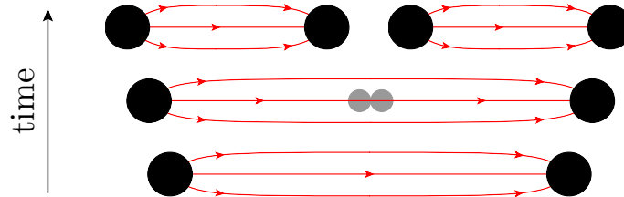
Figure 35.2: Illustration of string breaking by quark pair-creation in the string field.
