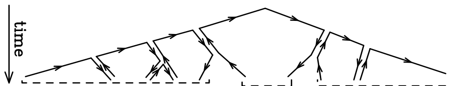
Figure 35.1: Color development of a shower in e^+e^- annihilation. Systems of color-connected partons are indicated by the dashed lines.
