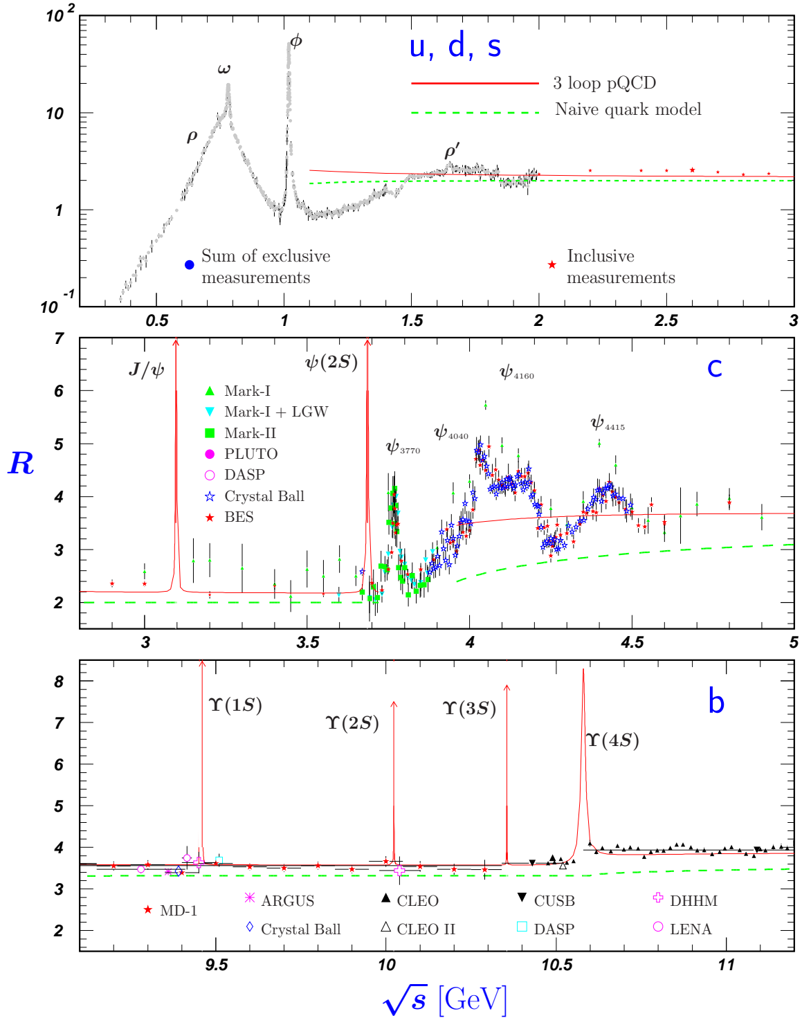
Figure 44.7: R in the light-flavor, charm, and beauty threshold regions. Data errors are total below 2 GeV and statistical above 2 GeV. The curves are the same as in Fig. 44.6. Note: CLEO data above \Upsilon(4S) were not fully corrected for radiative effects, and we retain them on the plot only for illustrative purposes with a normalization factor of 0.8. The full list of references to the original data and the details of the R ratio extraction from them can be found in [arXiv:hep-ph/0312114]. The computer-readable data are available at http://pdg.lbl.gov/current/xsect/ . (Courtesy of the COMPAS (Protvino) and HEPDATA (Durham) Groups, May 2010.)
