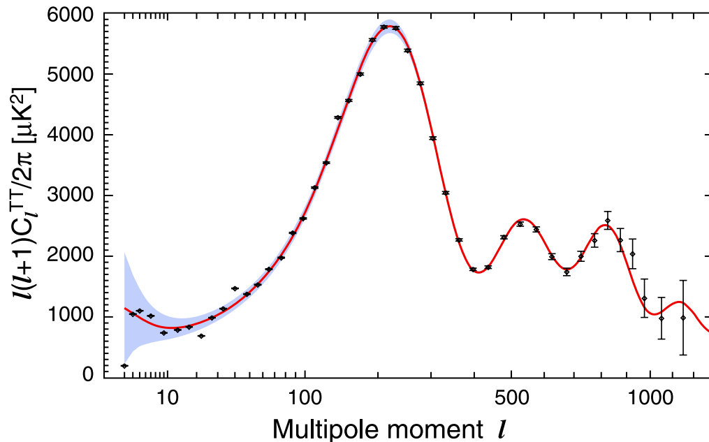
Figure 23.2: The angular power spectrum of the CMB temperature anisotropies from WMAP7, from Ref. 2. The grey band indicates the cosmic variance uncertainty. The solid line shows the prediction from the best-fitting \Lambda CDM model. [Figure courtesy NASA/WMAP Science Team.]
