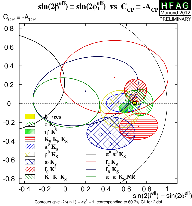
Figure 12.3: Summary of the results [25] of time-dependent analyses of b \rightarrow q\bar{q}s decays, which are potentially sensitive to new physics.
