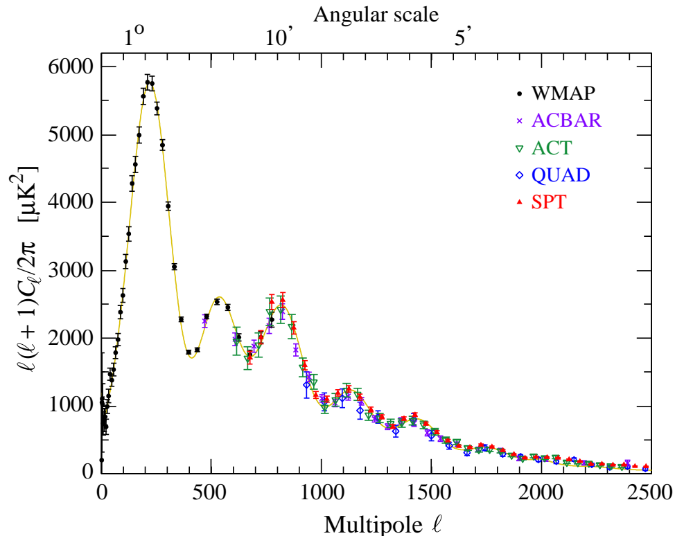
Figure 25.2: Band-power estimates from the WMAP, ACBAR, ACT, QUAD, and SPT experiments (omitting some band-powers which have larger error bars). Note that the widths of the \ell -bands vary between experiments and have not been plotted. This figure represents only a selection of available experimental results, with some other data-sets being of similar quality. The multipole axis here is linear, so the Sachs-Wolfe plateau is hard to see. However, the acoustic peaks and damping region are very clearly observed, with no need for a theoretical curve to guide the eye; the curve plotted is a best-fit model from WMAP plus other CMB data. At high \ell there is some departure from the model due to secondary anisotropies.
