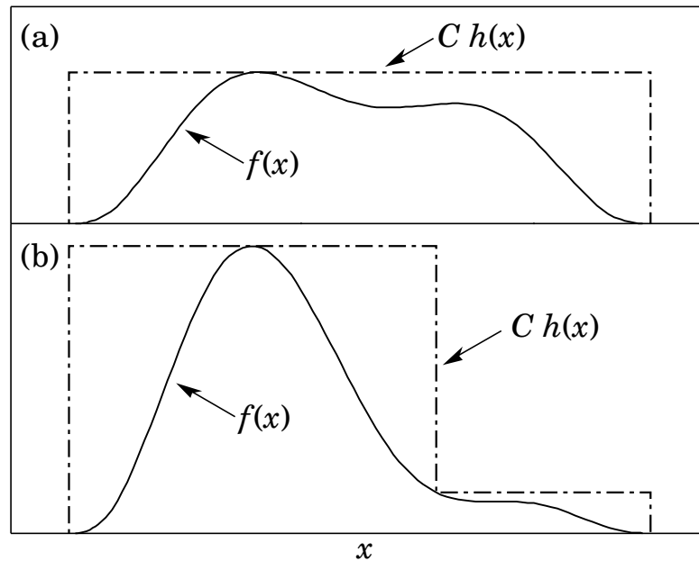
Figure 37.2: Illustration of the acceptance-rejection method. Random points are chosen inside the upper bounding figure, and rejected if the ordinate exceeds f(x) . The lower figure illustrates a method to increase the efficiency (see text).
