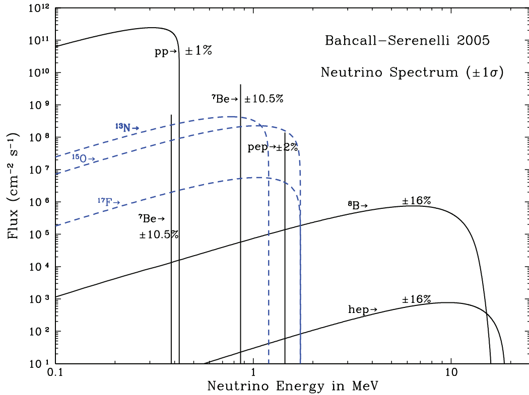
Figure 13.2: The solar neutrino spectrum predicted by the BS05(OP) standard solar model [102]. The neutrino fluxes are given in units of \text{cm}^{-2}\text{s}^{-1}\text{MeV}^{-1} for continuous spectra and \text{cm}^{-2}\text{s}^{-1} for line spectra. The numbers associated with the neutrino sources show theoretical errors of the fluxes. This figure is taken from the late John Bahcall's web site, http://www.sns.ias.edu/~jnb/ .
