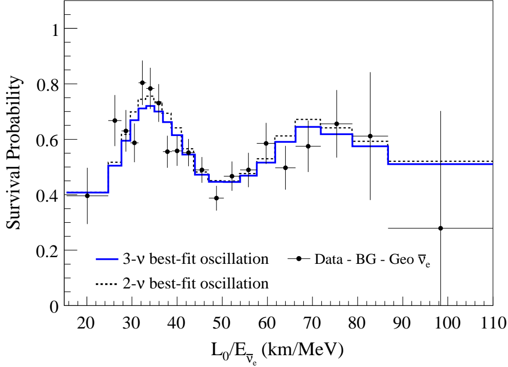
Figure 13.4: The ratio of the background and geoneutrino-subtracted \bar{\nu}_e spectrum, observed in the KamLAND experiment, to the predicted one without oscillations (survival probability) as a function of L_0/E , where L_0=180 km. The histograms show the expected distributions based on the best-fit parameter values from the two- and three-flavor neutrino oscillation analyses. The figure is from Ref. 129.
