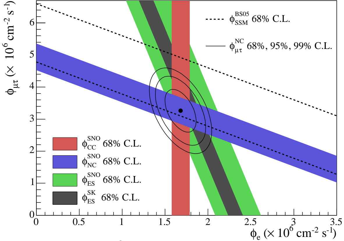
Figure 13.3: Fluxes of ^8\text{B} solar neutrinos, \phi(\nu_e) , and \phi(\nu_\mu \text{ or } \tau) , deduced from the SNO's CC, ES, and NC results of the salt phase measurement [116]. The Super-Kamiokande ES flux is from Ref. 126. The BS05(OP) standard solar model prediction [102] is also shown. The bands represent the 1\sigma error. The contours show the 68%, 95%, and 99% joint probability for \phi(\nu_e) and \phi(\nu_\mu \text{ or } \tau) . The figure is from Ref. 116.
