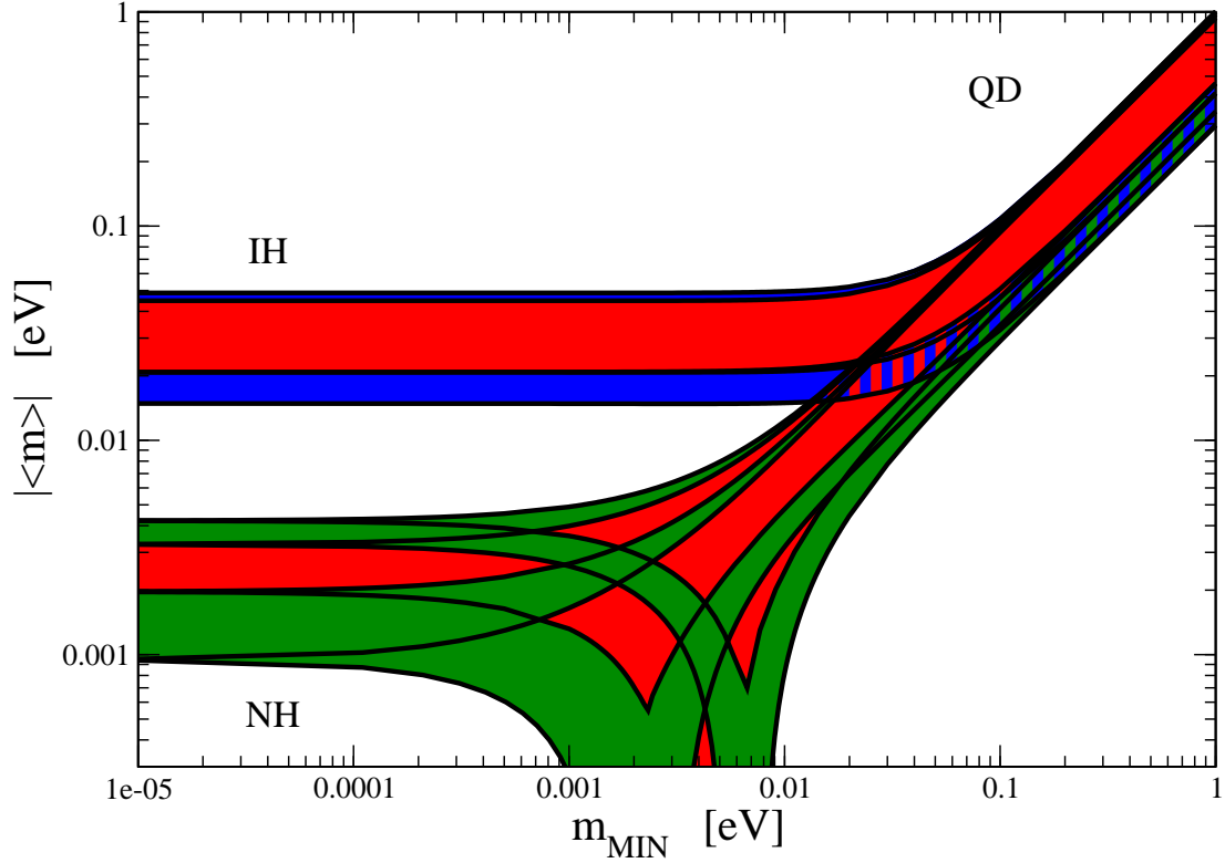
Figure 13.10: The effective Majorana mass |\langle m \rangle| (including a 2\sigma uncertainty), as a function of \min(m_j) for \sin^2 \theta_{13} = 0.0236 \pm 0.0042 [31] and \delta = 0 . The figure is obtained using also the best fit values and 1\sigma errors of \Delta m_{21}^2 , \sin^2 \theta_{12} , and |\Delta m_{31}^2| \cong |\Delta m_{32}^2| from Ref. 196. For \sin^2 \theta_{12} the results found with the “old” reactor \bar{\nu}_e fluxes [159] were employed. The phases \alpha_{21,31} are varied in the interval [0, \pi] . The predictions for the NH, IH and QD spectra are indicated. The red regions correspond to at least one of the phases \alpha_{21,31} and (\alpha_{31} - \alpha_{21}) having a CP violating value, while the blue and green areas correspond to \alpha_{21,31} possessing CP conserving values. (Update by S. Pascoli of a figure from the last article quoted in Ref. 195.)
