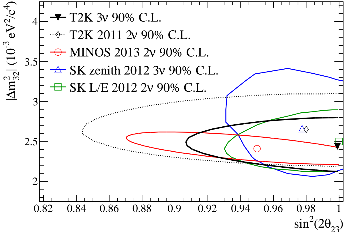
Figure 13.6: The 90% CL allowed regions from \nu_\mu disappearance results: T2K 2013 [23], T2K2011 [22], Super-Kamiokande [136], and MINOS [143]. The MINOS contour was obtained by assuming identical neutrino and antineutrino oscillation parameters. This figure is taken from Ref. 23.
