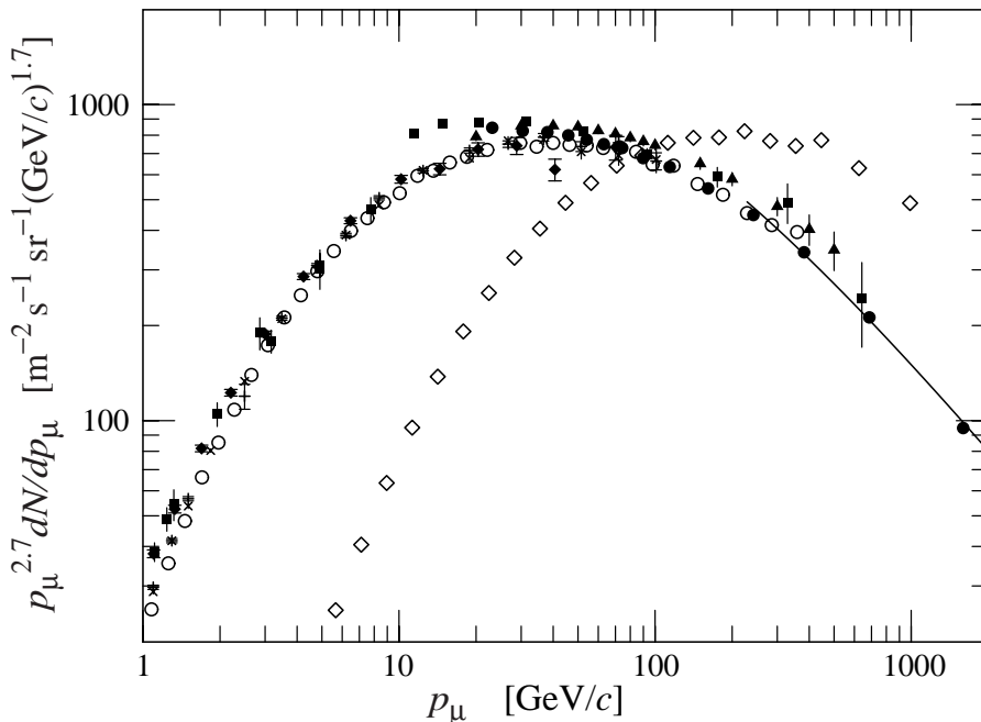
Figure 28.5: Spectrum of muons at \theta = 0^\circ ( \diamond [48], \blacksquare [54], \blacktriangledown [55], \blacktriangle [56], \times , + [50], \circ [51], and \bullet [52] and \theta = 75^\circ \diamond [57]). The line plots the result from Eq. (28.4) for vertical showers.
