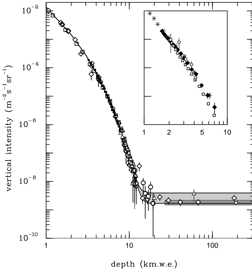
Figure 28.7: Vertical muon intensity vs depth (1 km.w.e. = 10^5 g \text{cm}^{-2} of standard rock). The experimental data are from: \diamond : the compilations of Crouch [67], \square : Baksan [72], \circ : LVD [73], \bullet : MACRO [74], \blacksquare : Frejus [75], and \triangle : SNO [76]. The shaded area at large depths represents neutrino-induced muons of energy above 2 GeV. The upper line is for horizontal neutrino-induced muons, the lower one for vertically upward muons. Darker shading shows the muon flux measured by the SuperKamiokande experiment. The inset shows the vertical intensity curve for water and ice published in Refs. [68–71].
