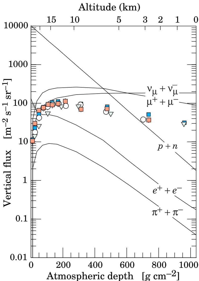
Figure 28.4: Vertical fluxes of cosmic rays in the atmosphere with E > 1 GeV estimated from the nucleon flux of Eq. (28.2). The points show measurements of negative muons with E_\mu > 1 GeV [39–43].
