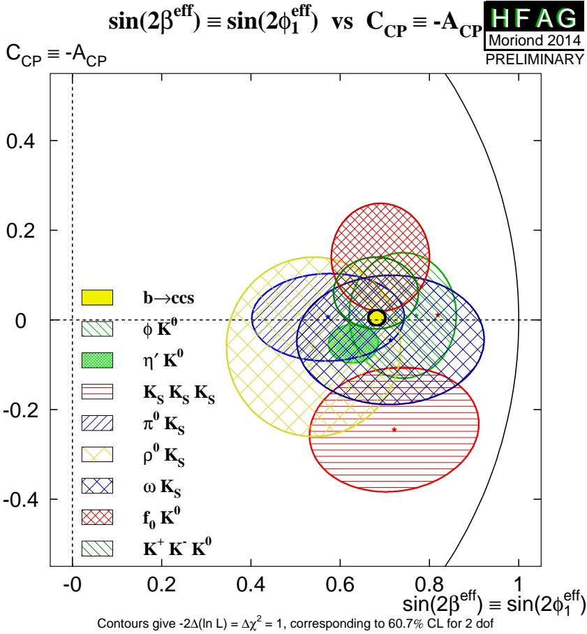
Figure 13.3: Summary of the results [27] of time-dependent analyses of b \rightarrow q\bar{q}s decays, which are potentially sensitive to new physics.
