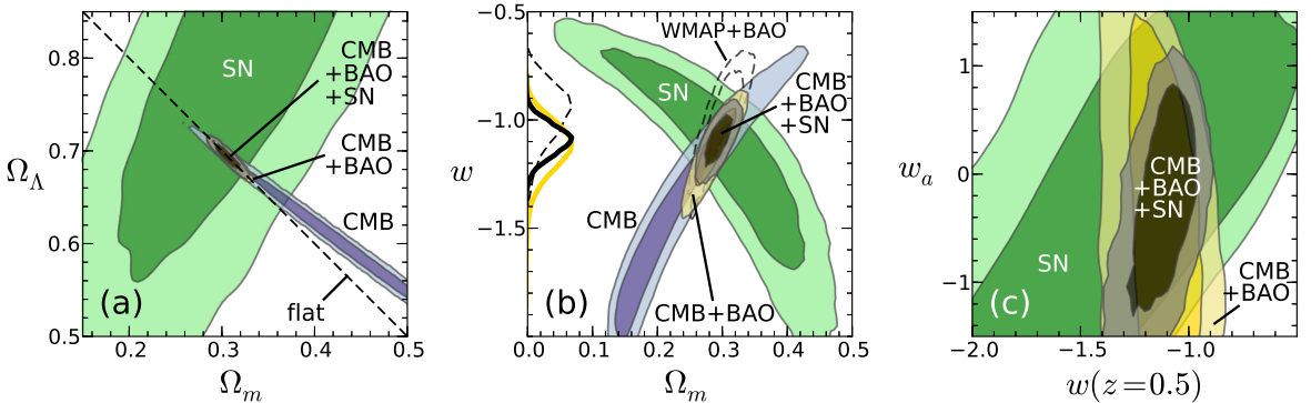
Figure 26.2: Constraints on the present matter fraction \Omega_m and dark energy model parameters. Dark and light shaded regions indicate 68.3% and 95.4% confidence levels, respectively. “CMB” is Planck+WP, “BAO” is the combination of SDSS-II, BOSS, and 6dFGS, and “SN” is Union2. (a) The present dark energy fraction \Omega_\Lambda vs. \Omega_m , assuming a \Lambda CDM model. CMB data, especially when combined with BAO constraints, strongly favor a flat universe (diagonal dashed line). (b) The dark energy equation of state w vs. \Omega_m , assuming a constant value of w . The dashed contours show the 68.3% and 95.4% CL regions for the combination of WMAP9 and BAO data. Curves on the left vertical axis show the probability distributions for w (normalized arbitrarily), after marginalizing over \Omega_m , for the CMB+BAO and CMB+BAO+SN combinations (yellow and black, respectively), using Planck+WP CMB data, and for the WMAP9+BAO combination (dashed black). (c) Constraints on the two parameters of the dark energy model with a time-dependent equation of state given by Eq. (26.4): w(z = 0.5) and w_a = -dw/da .
